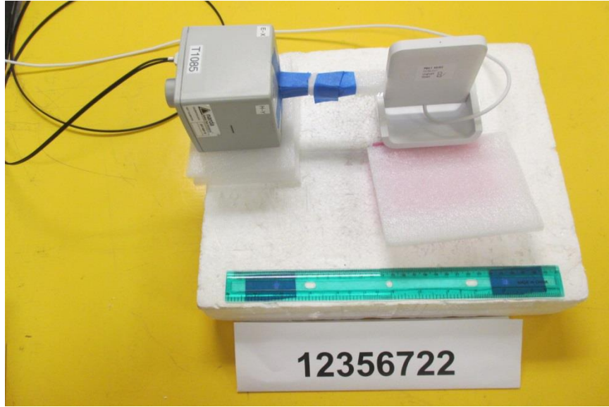
S3, RF EXPOSURE SETUP PHOTO
