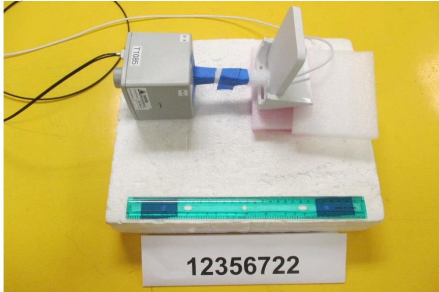
S4, RF EXPOSURE SETUP PHOTO
