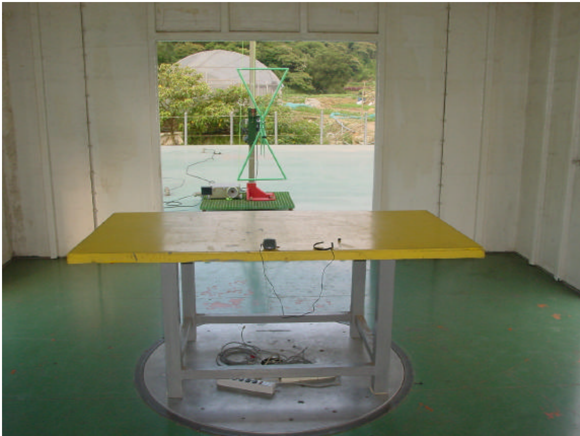
Radiated (30~1000MHz)
