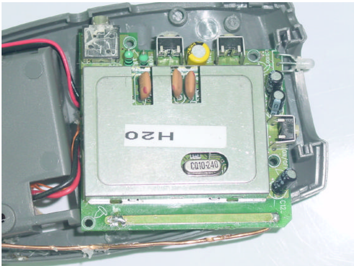
PCB (RF Module & Component Side)
