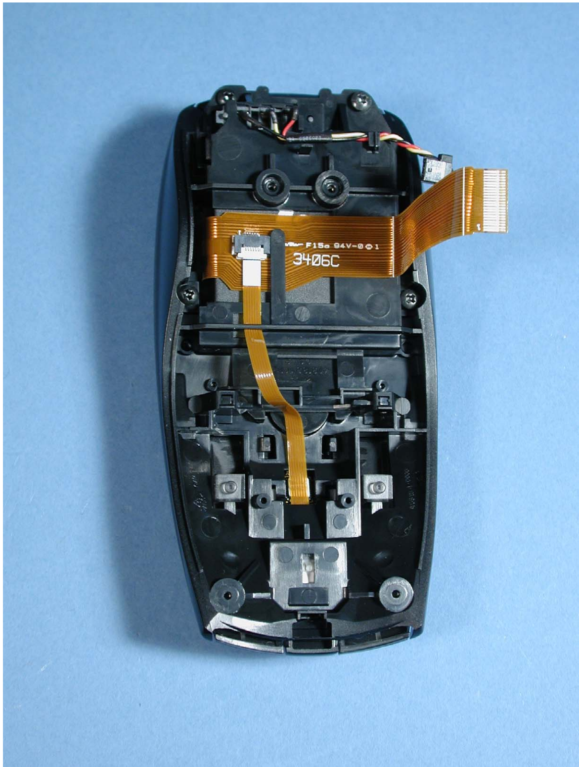
Photograph 1: M-RBP123 inside view of top part
