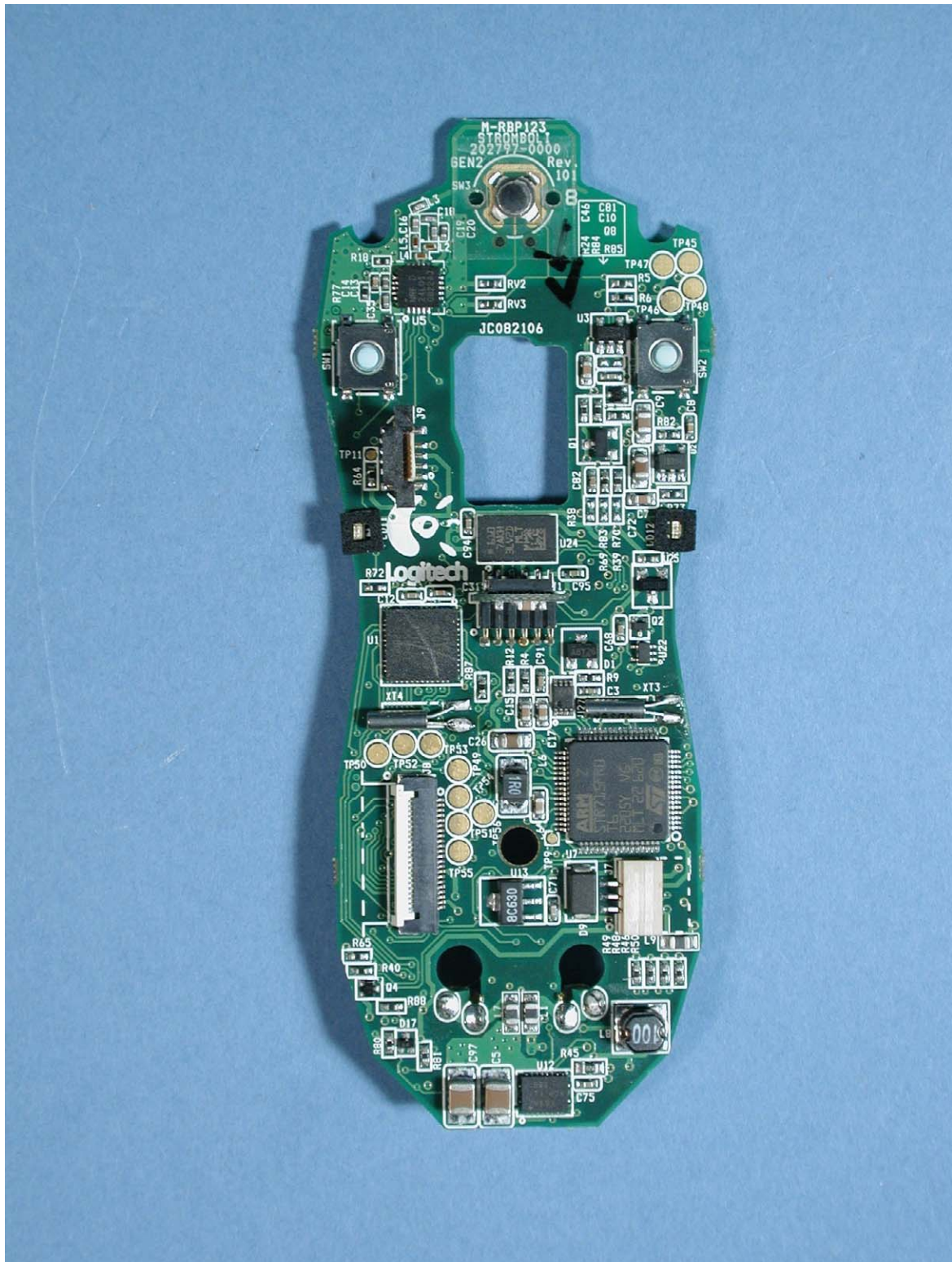
Photograph 3: PCB of M-RBP123 top view
