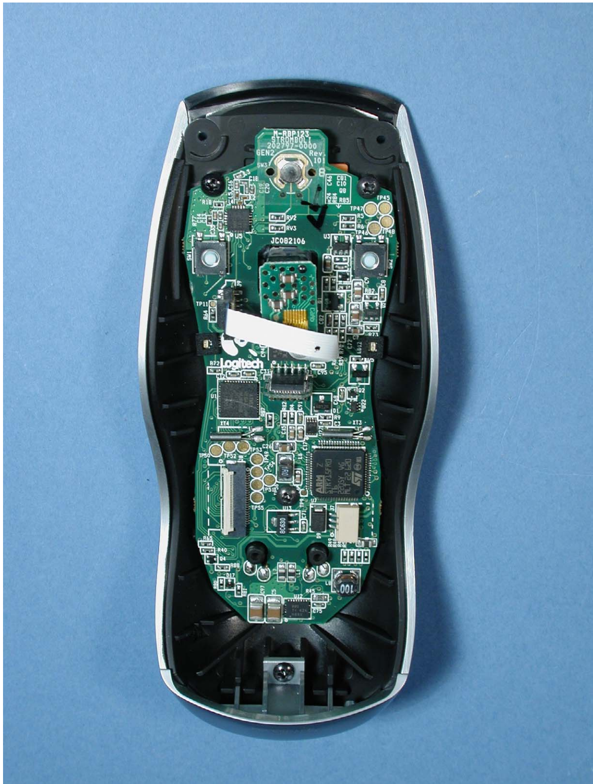
Photograph 2: M-RBP123 inside view of bottom part
