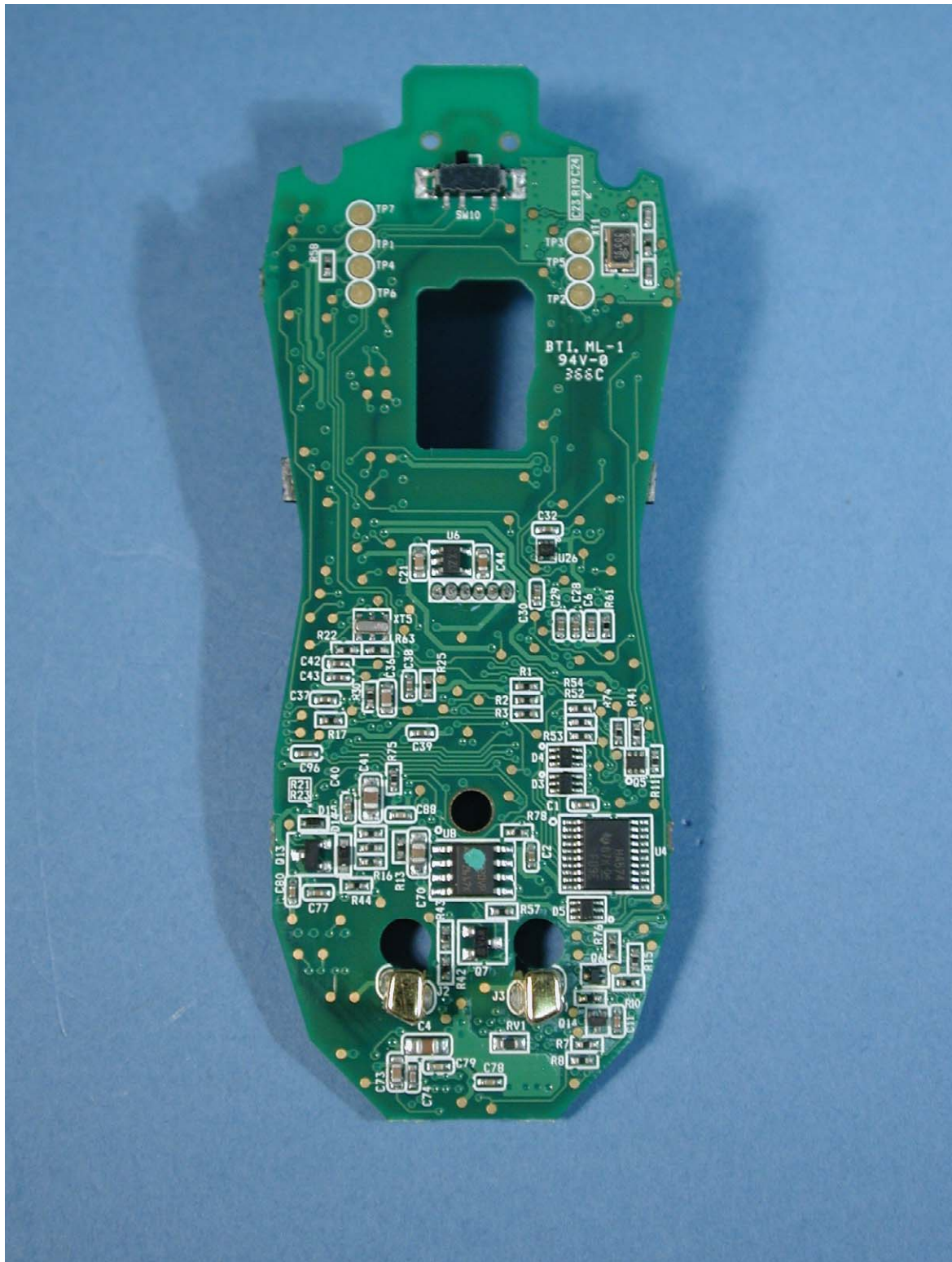
Photograph 4: PCB of M-RBP123 bottom view
