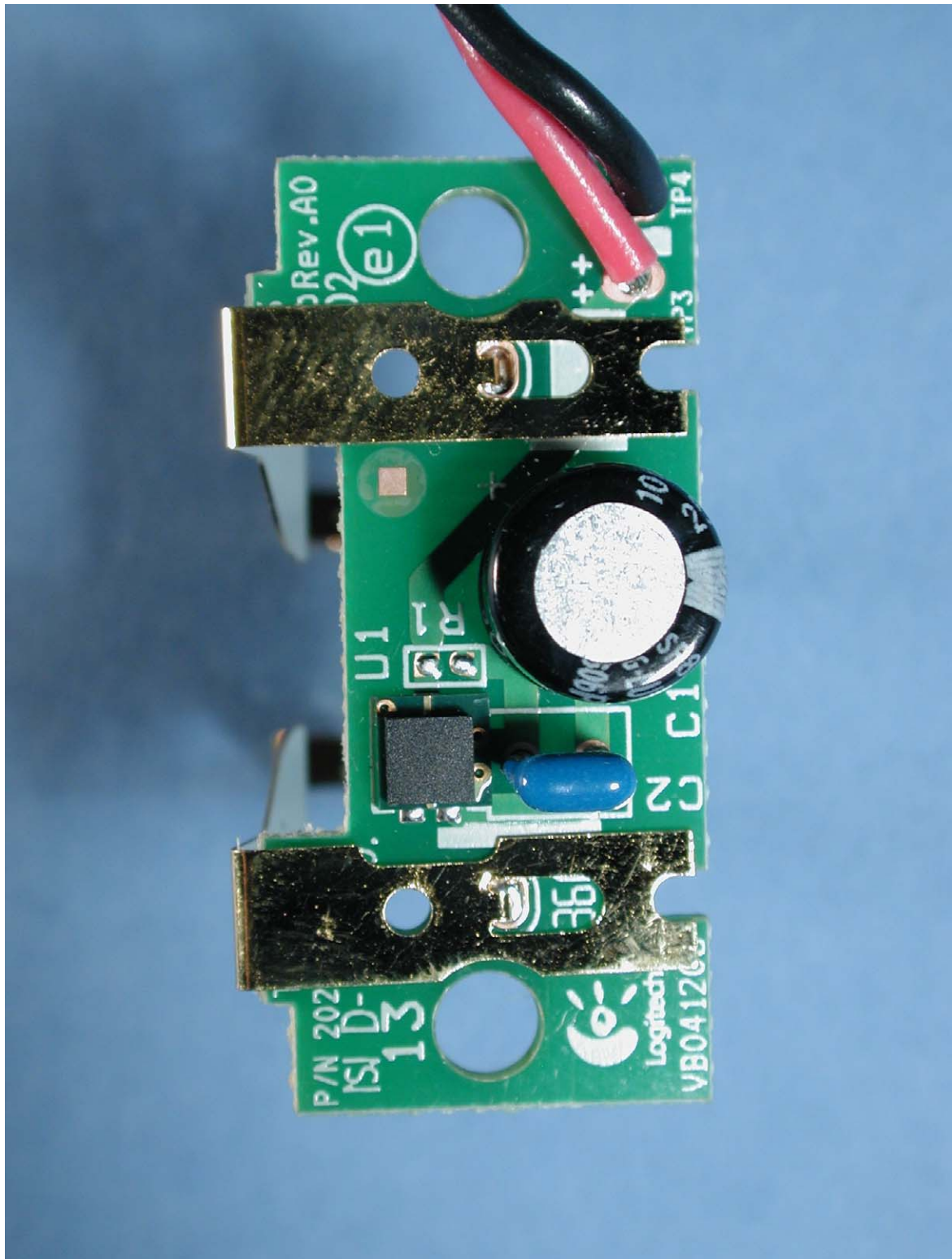
Photograph 7: PCB of cradle L-LM12, top view
