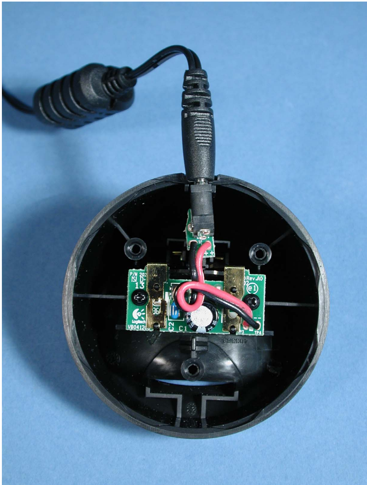
Photograph 5: Cradle L-LM12, interior view, top part
