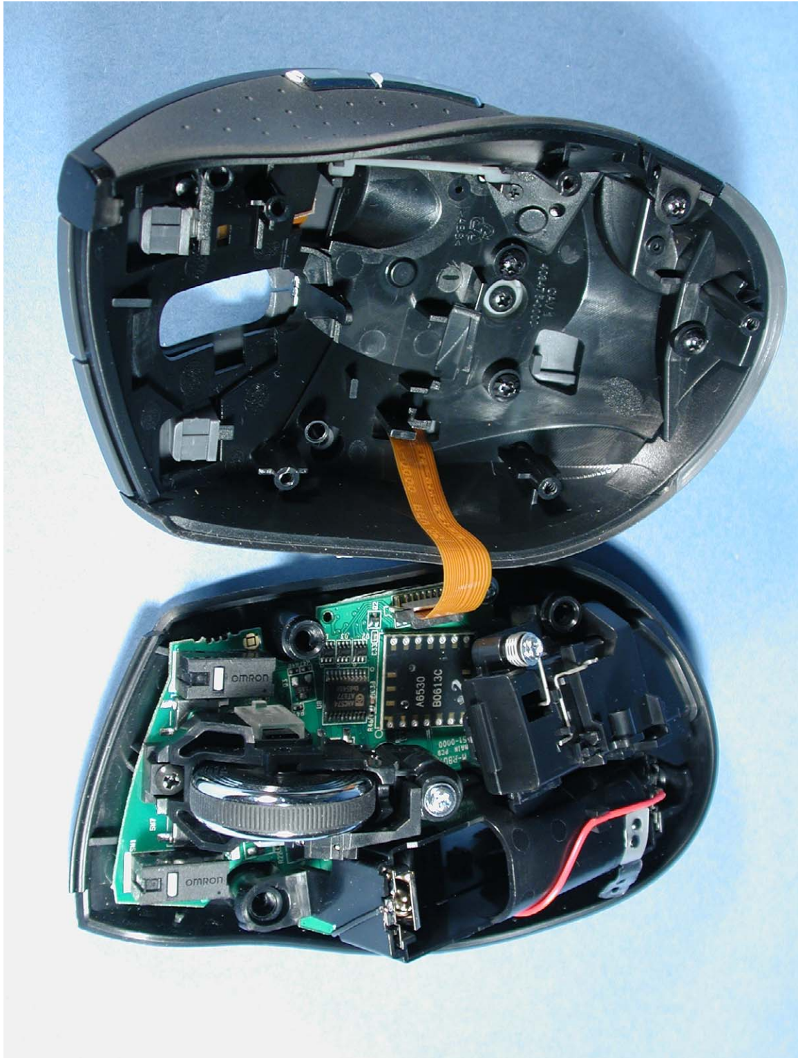
Photograph 1: M-RBU126, exploded view
