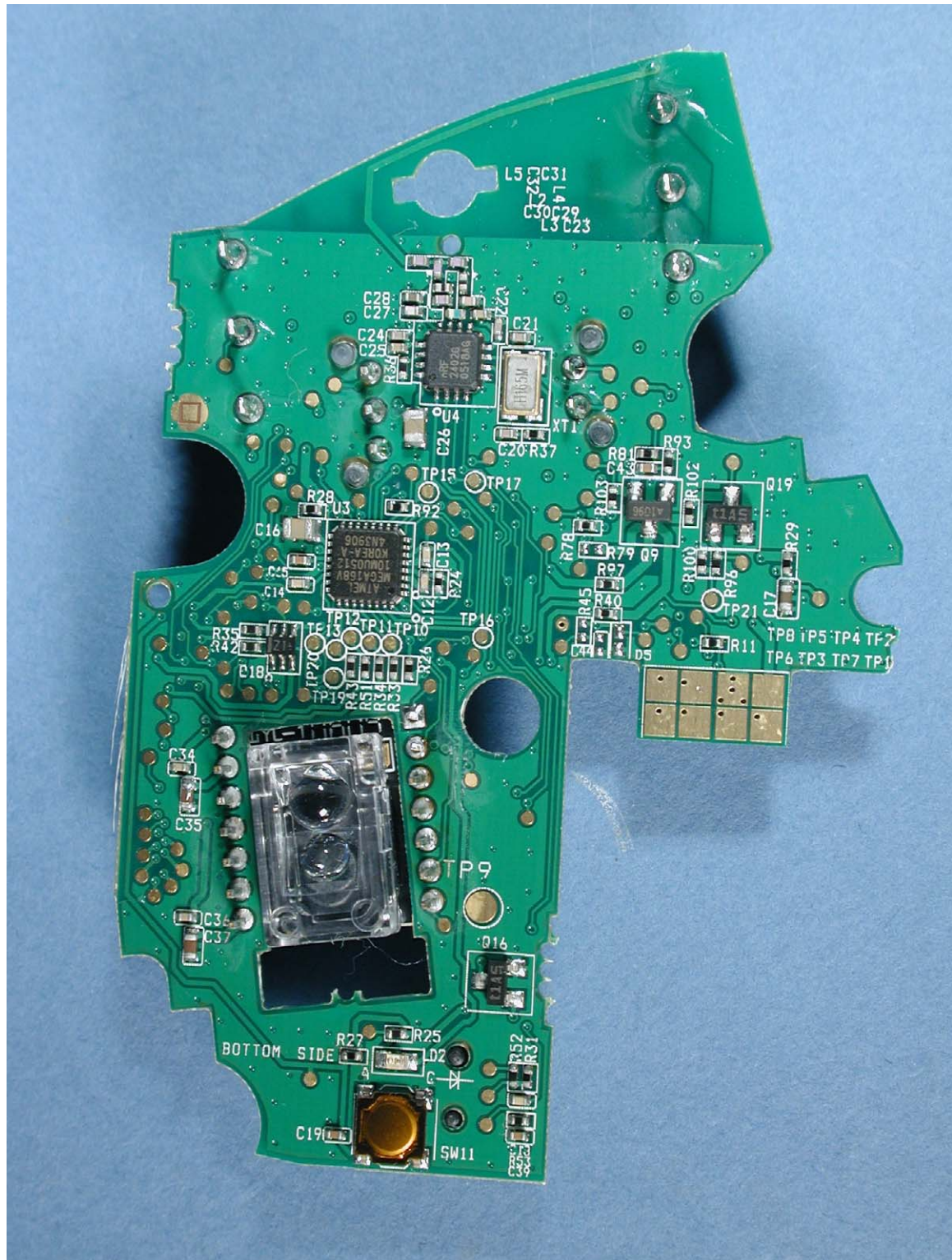
Photograph 3: M-RBU126, PCB bottom side
