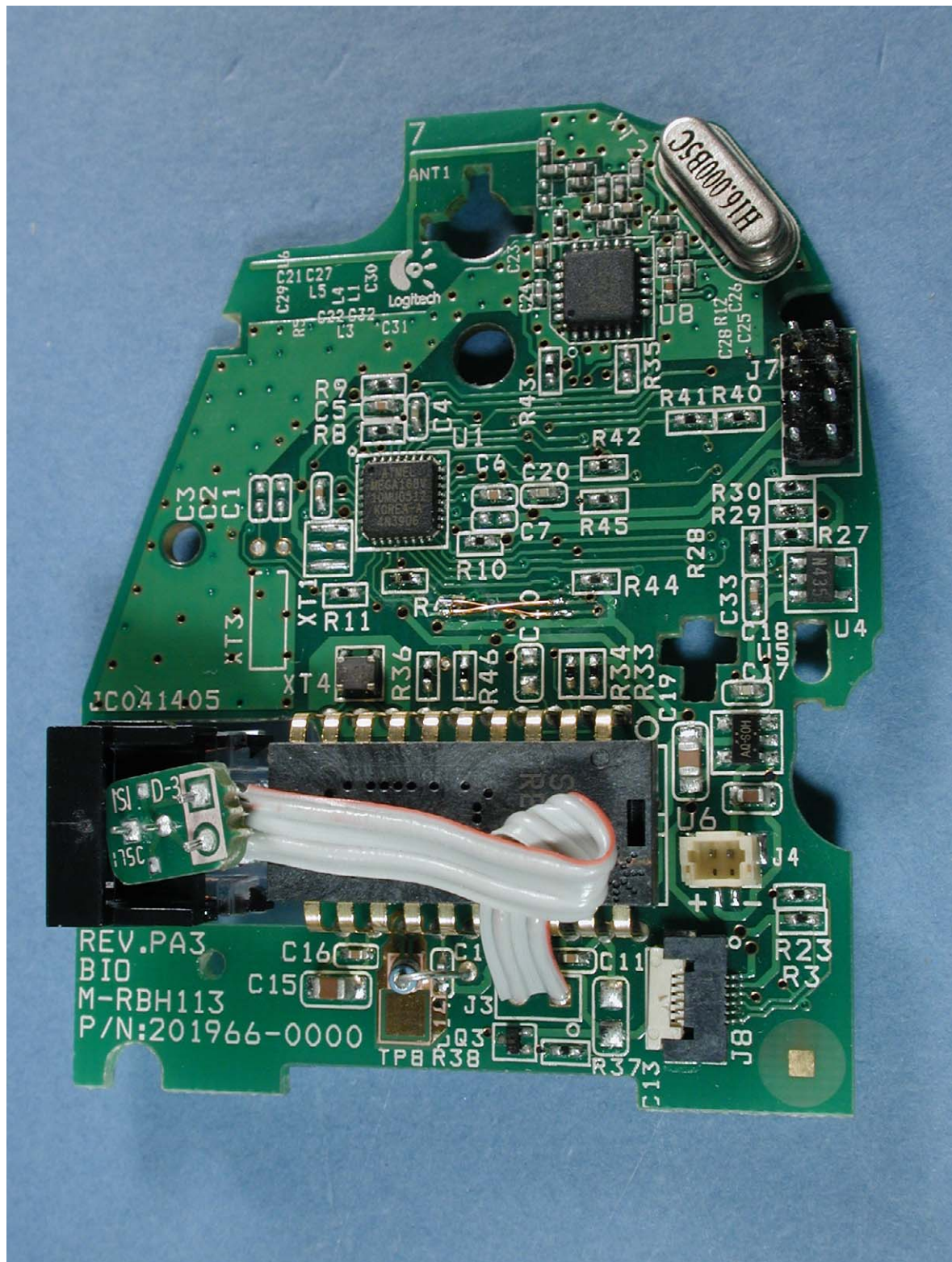
Photograph 8: M-RBH113 main PCB top view
