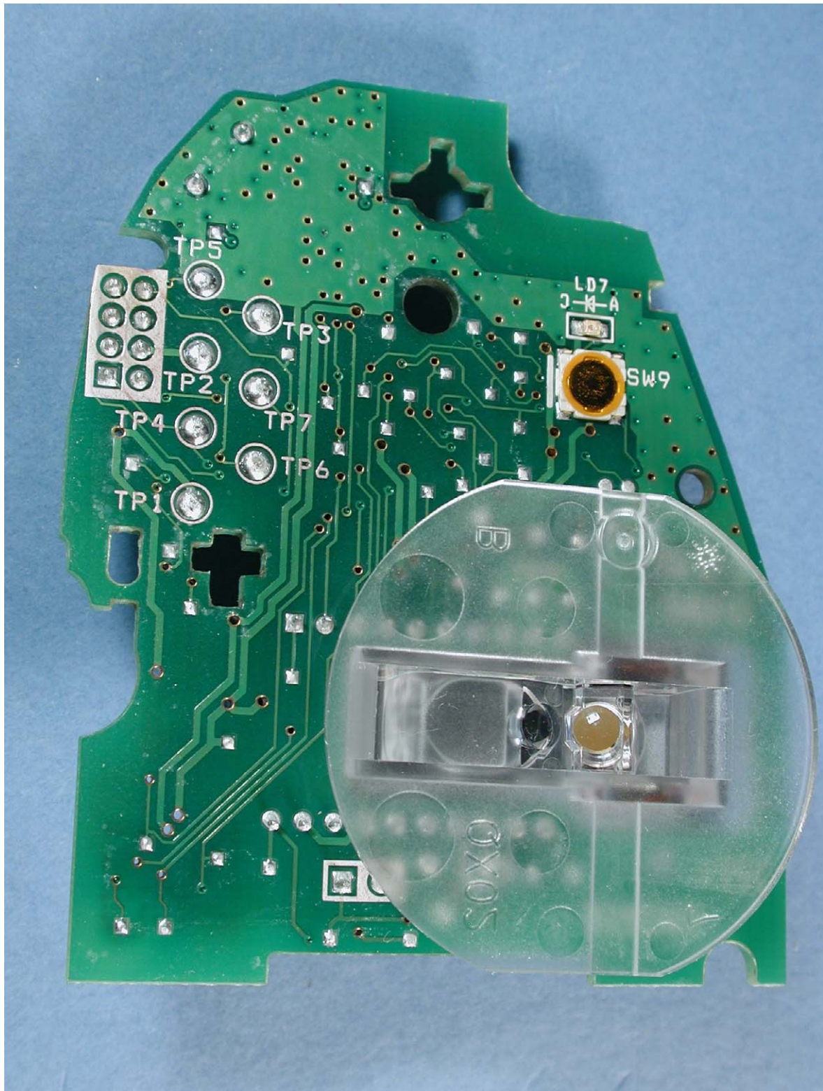
Photograph 9: M-RBH113 main PCB bottom view
