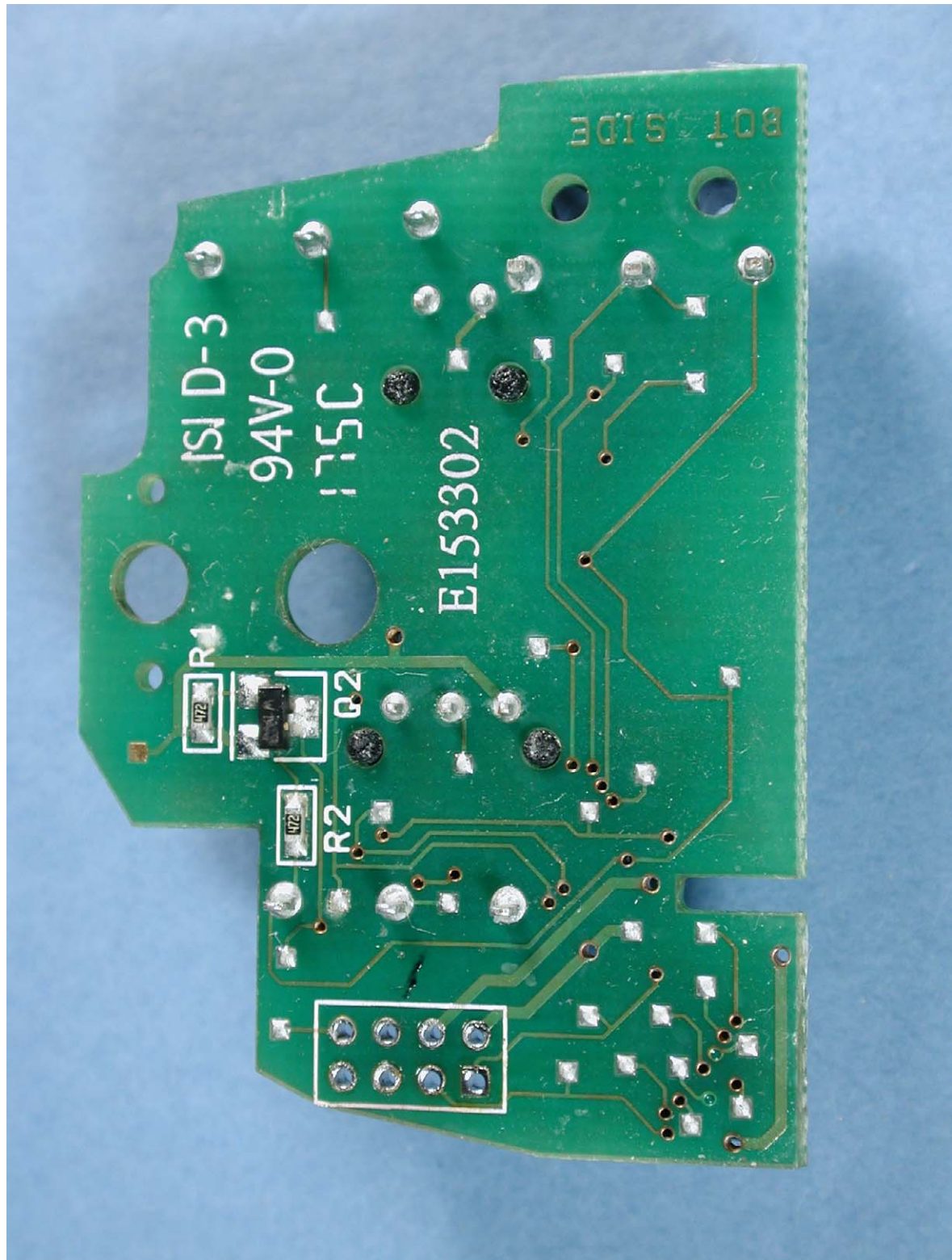
Photograph 7: M-RBH113 button PCB bottom view
