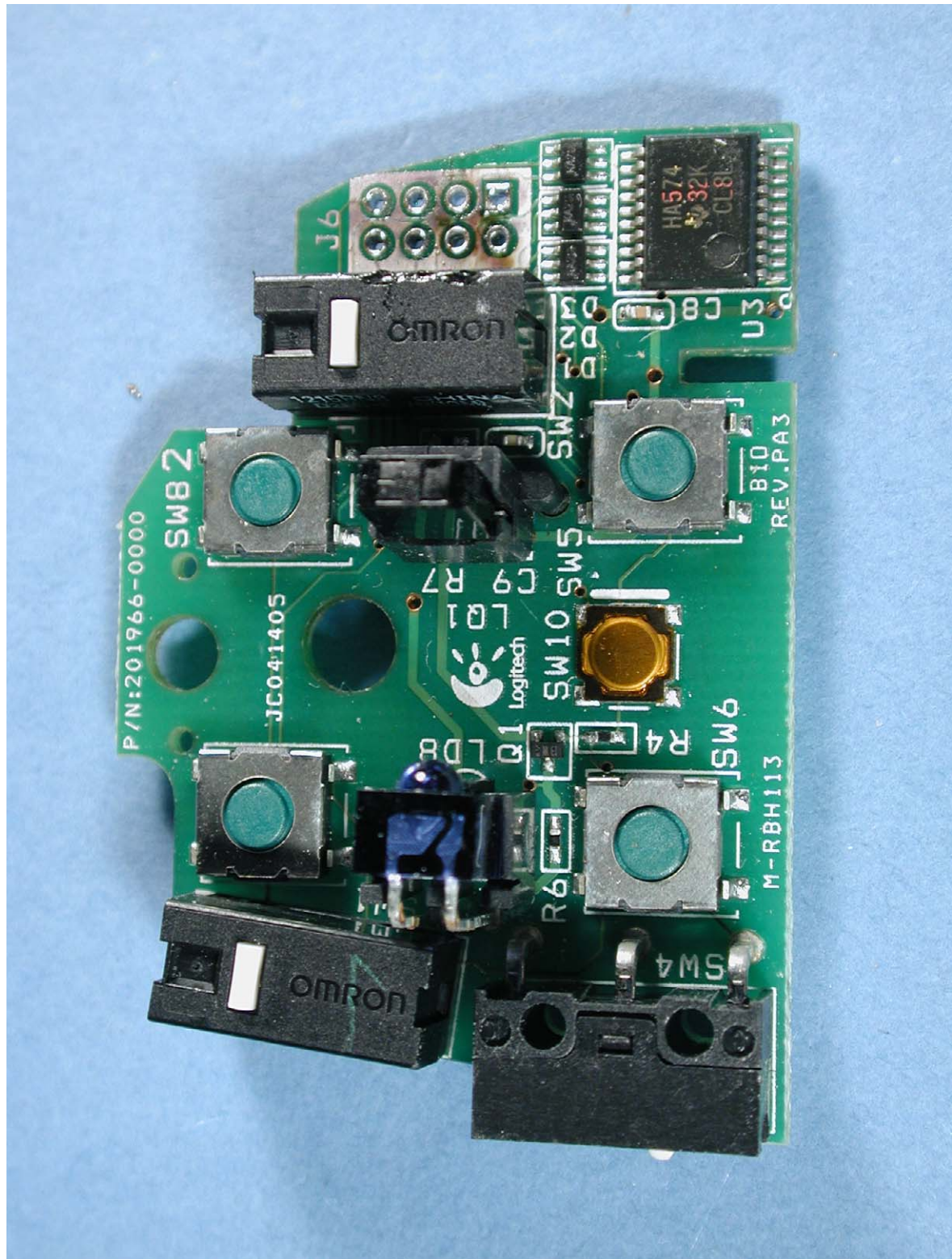
Photograph 6: M-RBH113 button PCB top view
