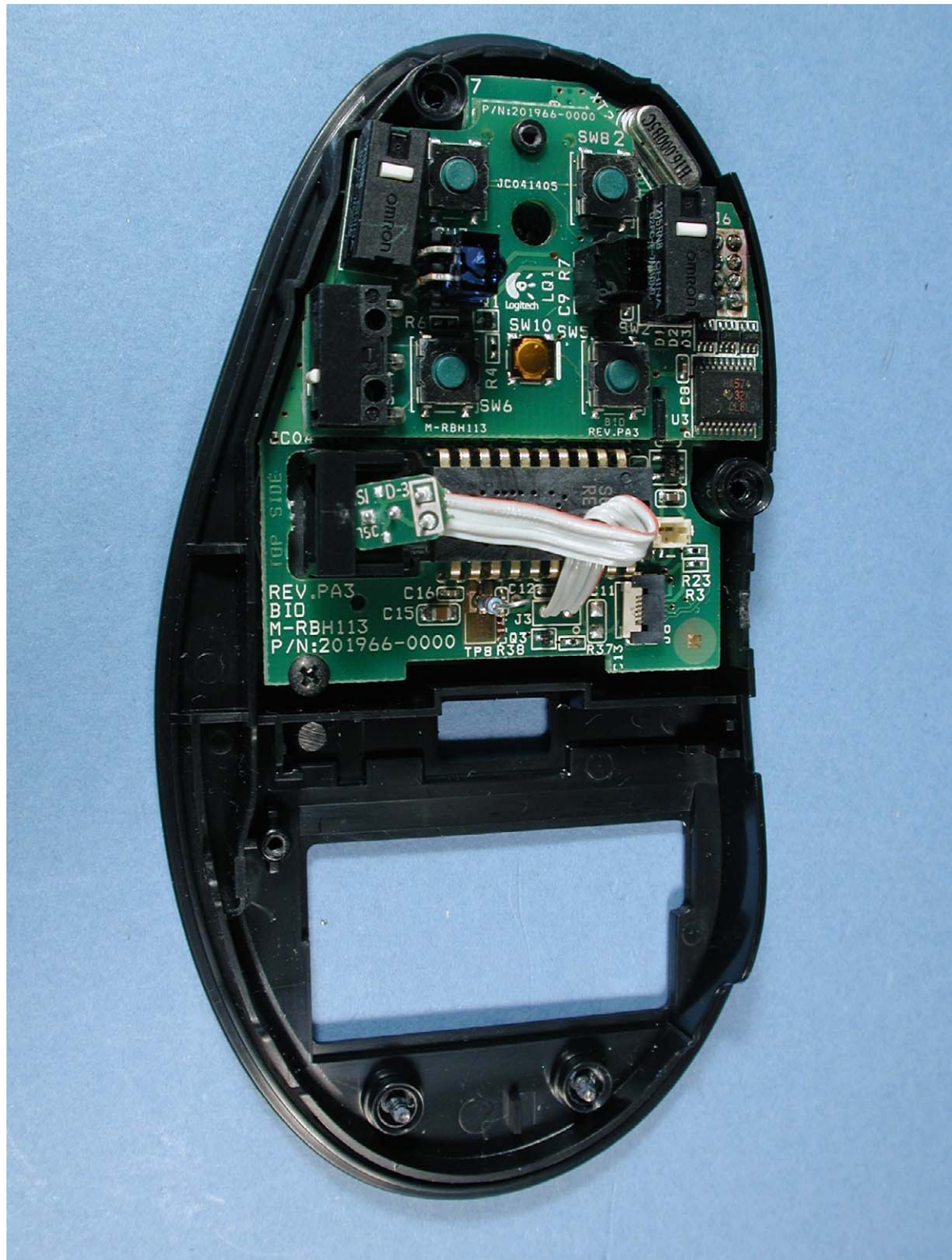
Photograph 4: M-RBH113 Base with PCB's without battery compartment
