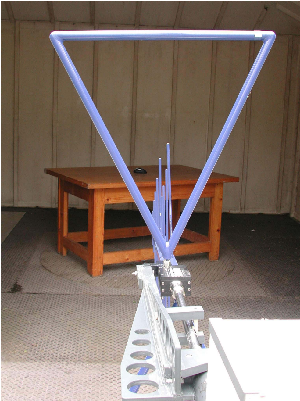
Photograph 3: Test set up: radiated emissions above 30 MHz at 3 m distance
