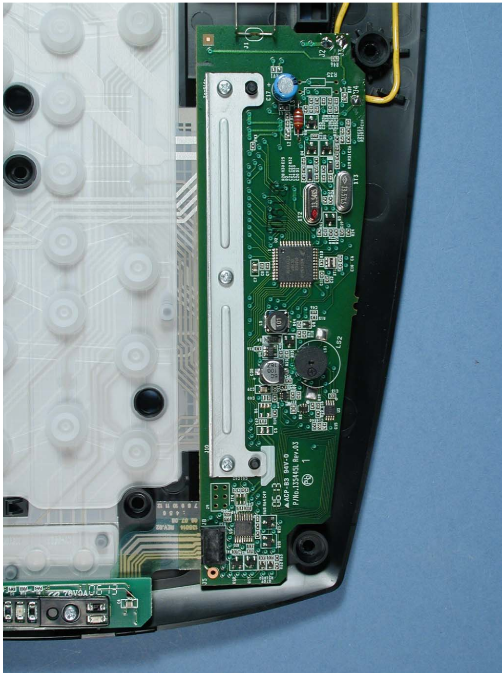
Photograph 3: Main PCB of Y-RAV80
