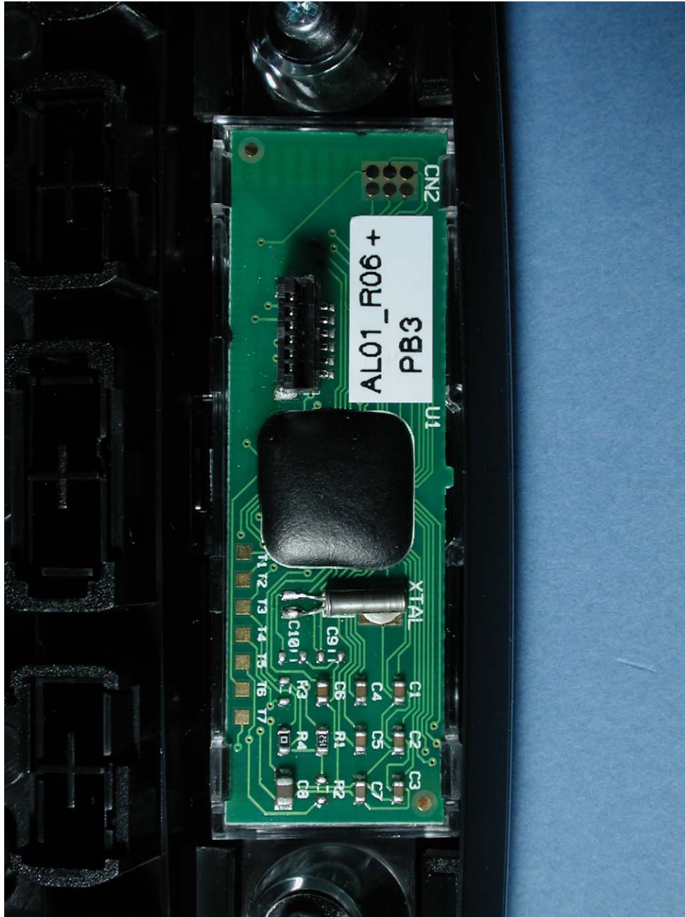
Photograph 4: Slider PCB of Y-RAV80
