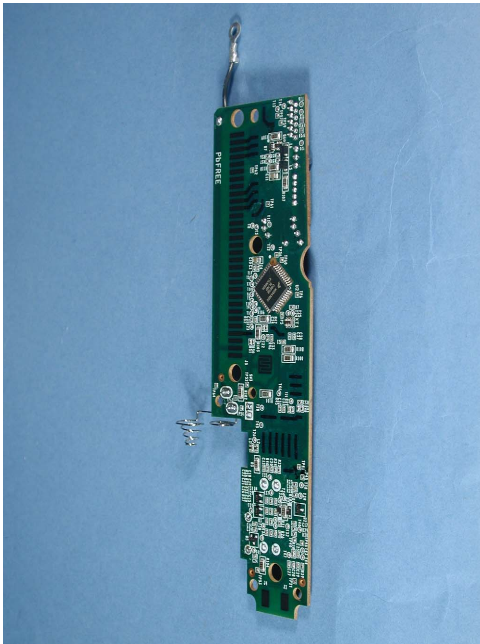
Photograph 6: Rear view PCB of Y-RAM74
