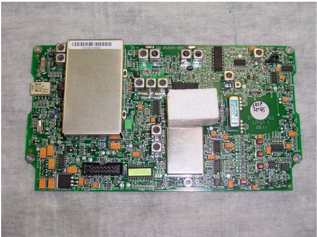
8. 2010 RF/IF assembly 08-05889-001
