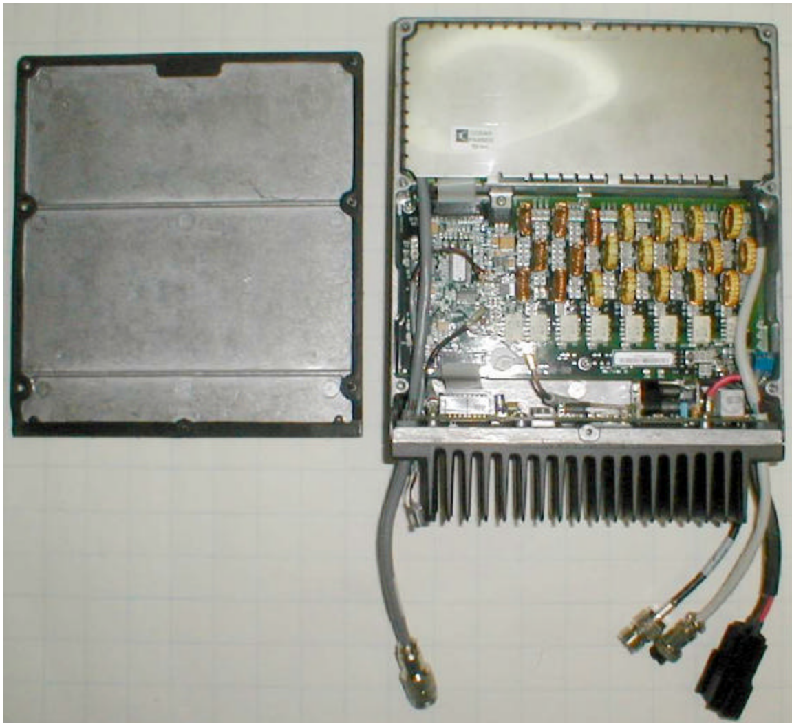
Top - Cover Removed
