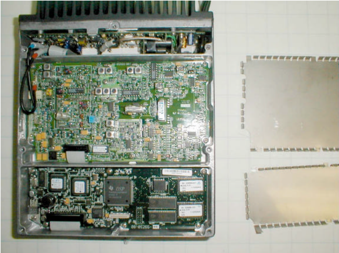
Bottom - Shields Removed
