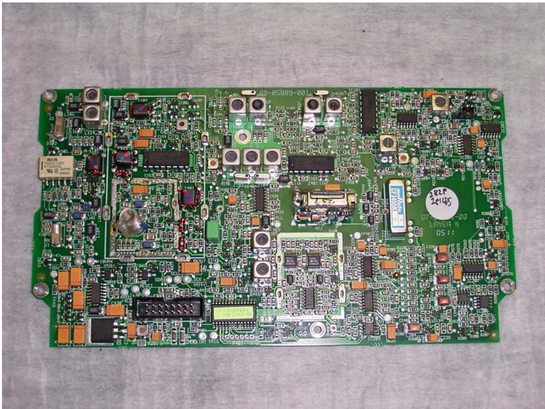
8. 2011 RF/IF assembly with all screens removed (08-05889-001)
