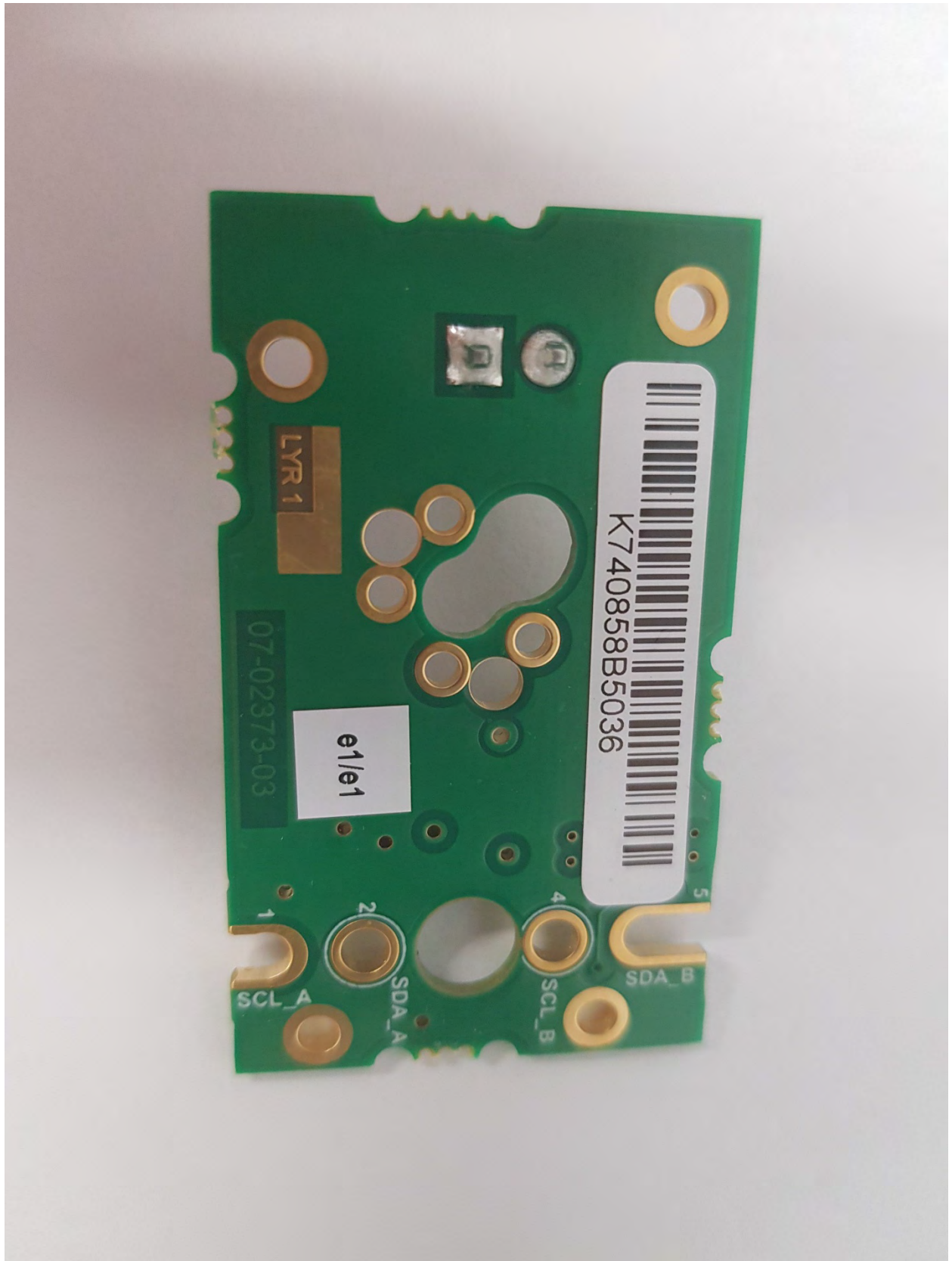
REAR PANEL PCB 08-07510 – 001 – SIDE 2
