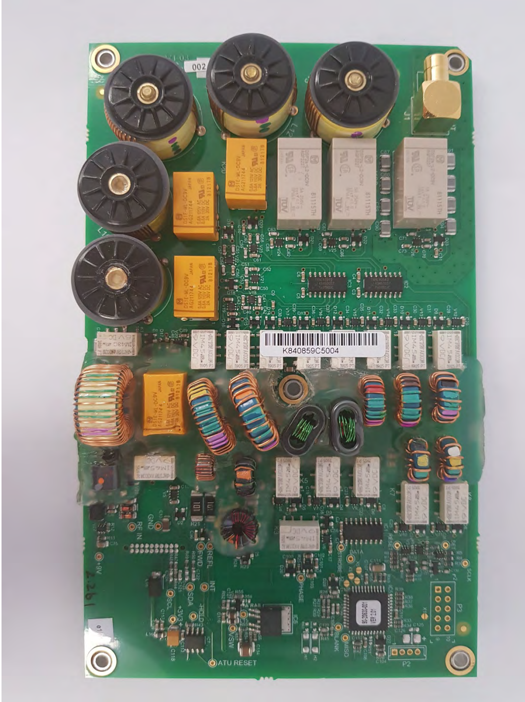
ANTENNA TUNER PCB 08-07508-002 – SIDE 1
