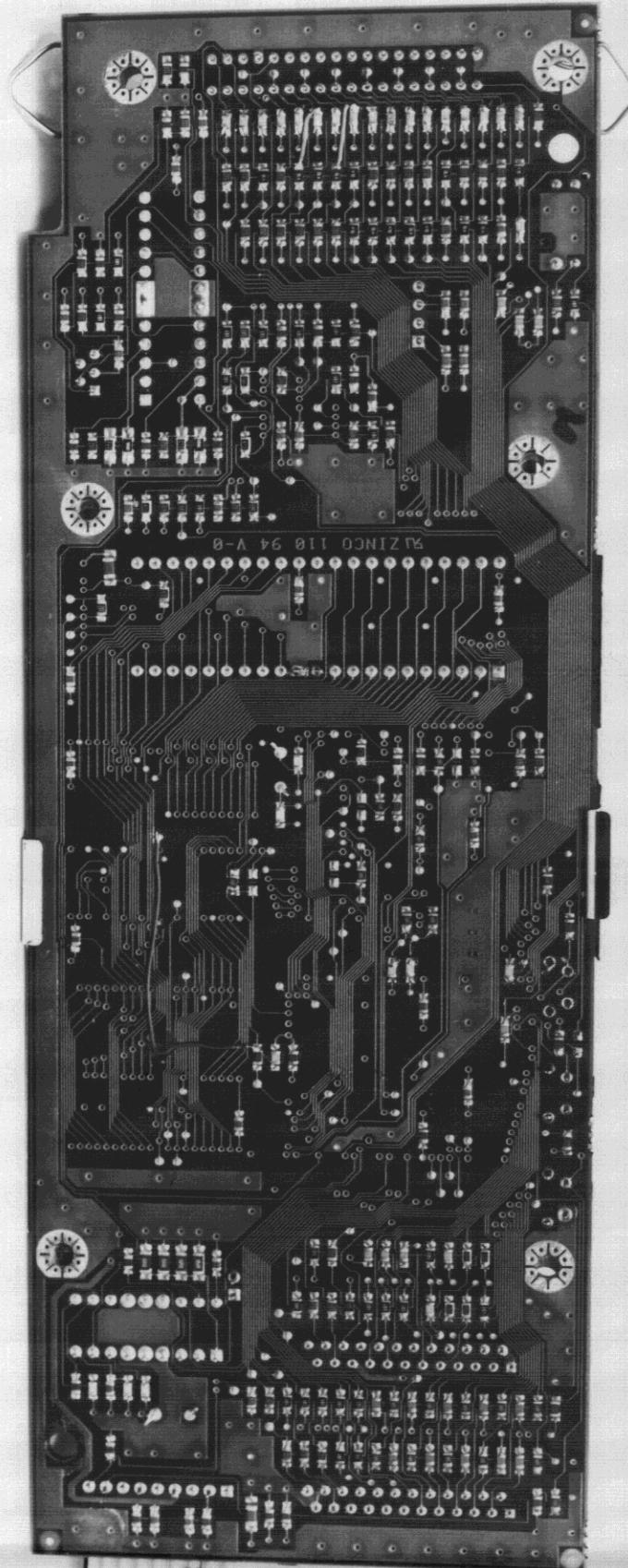
Fig. 8.8 Controller Board - Foil side
