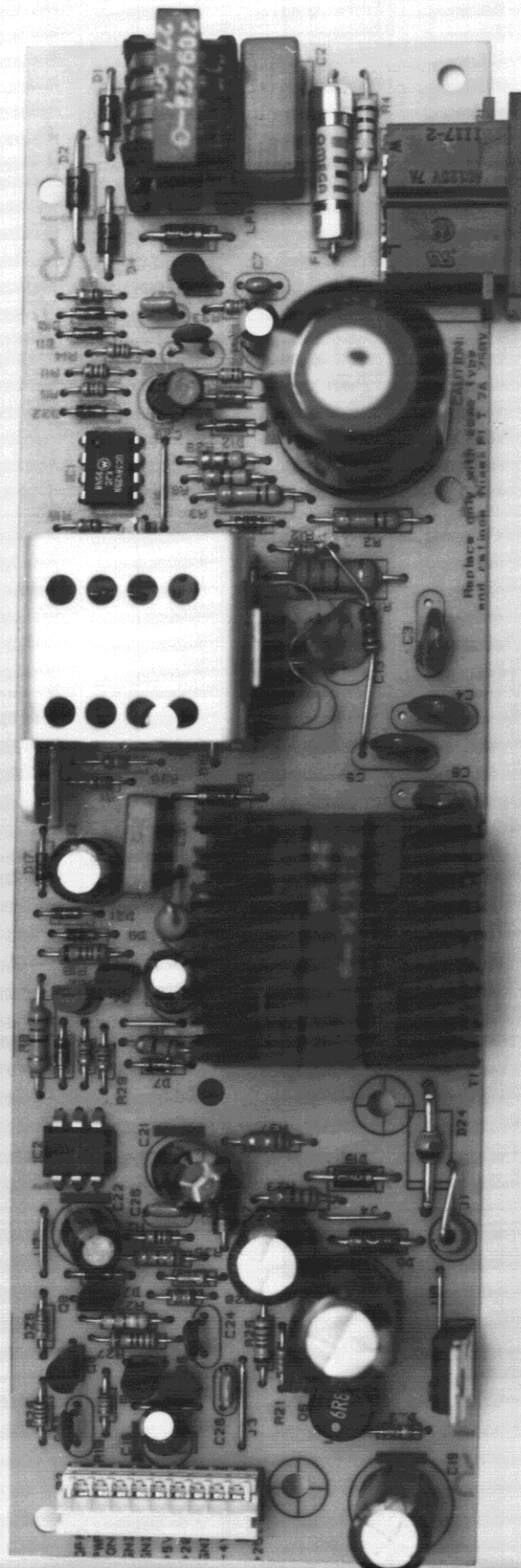
Fig. 8.5 Power Supply Unit P.W.A. - Components side
