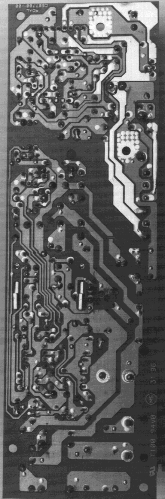
Fig. 8.6 Power Supply Unit P.W.A. - Foil side
