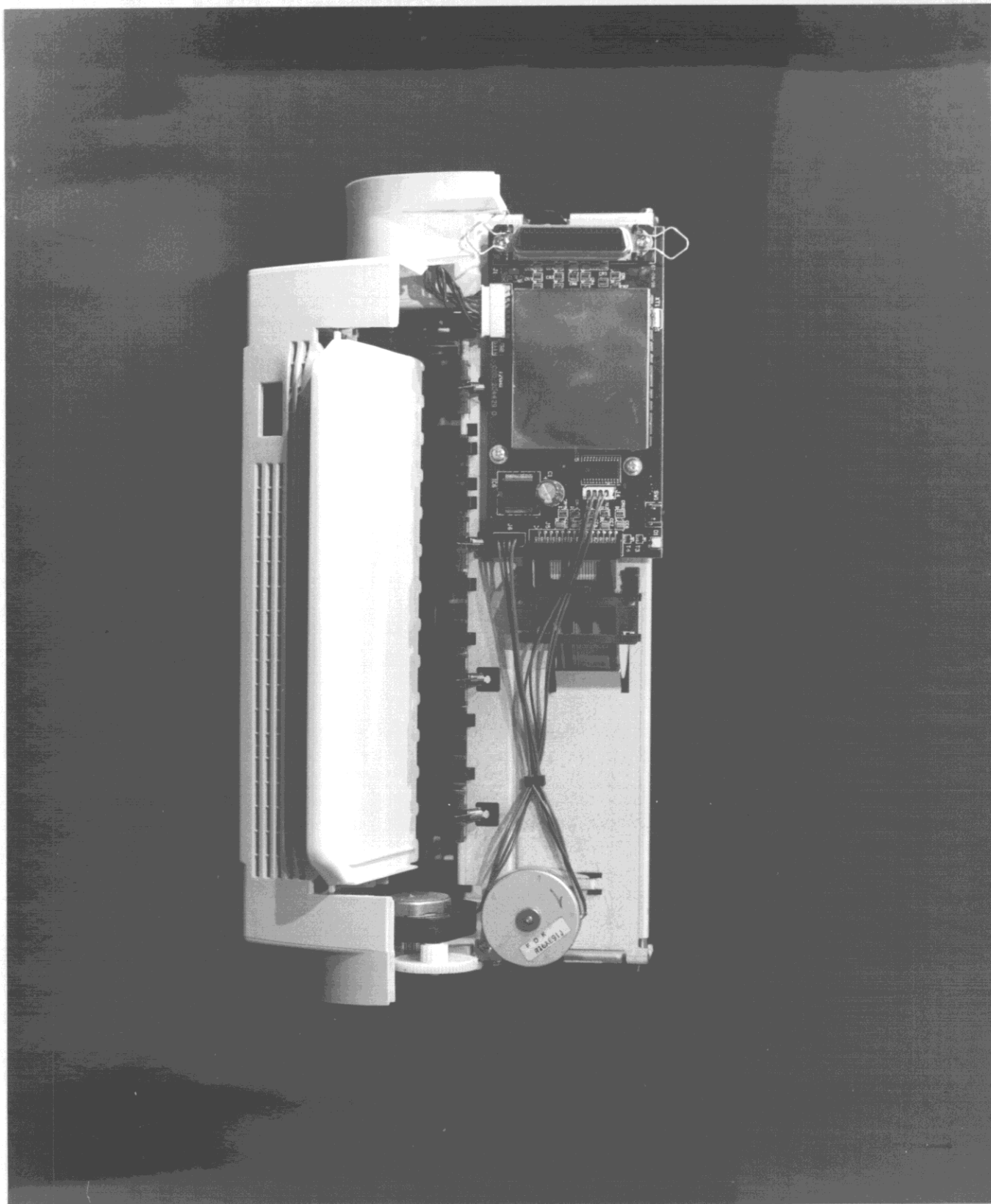
Fig. 8.4 Internal view with upper cover removed (without paper feeder)
