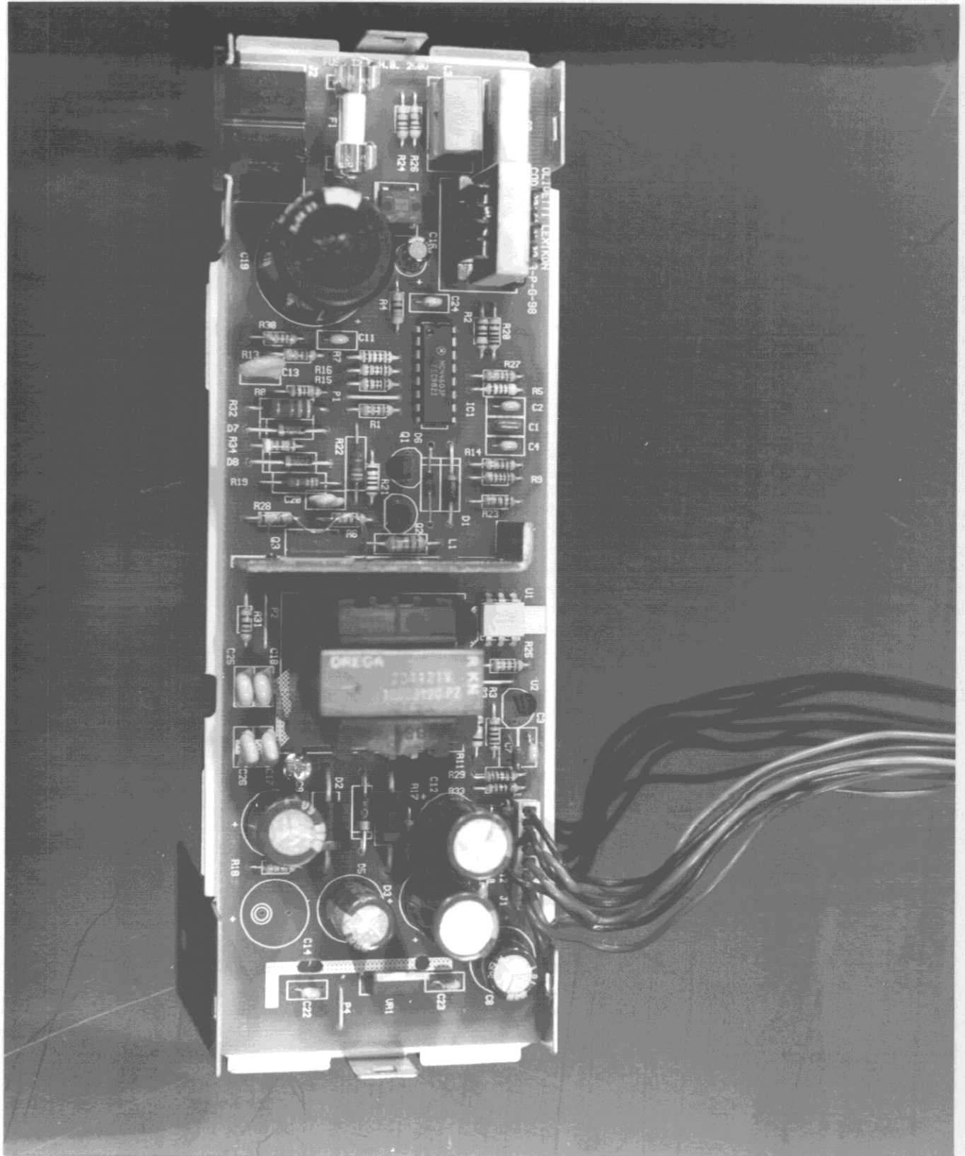
Fig. 8.5 Power Supply Unit P.W.A. - Components side
