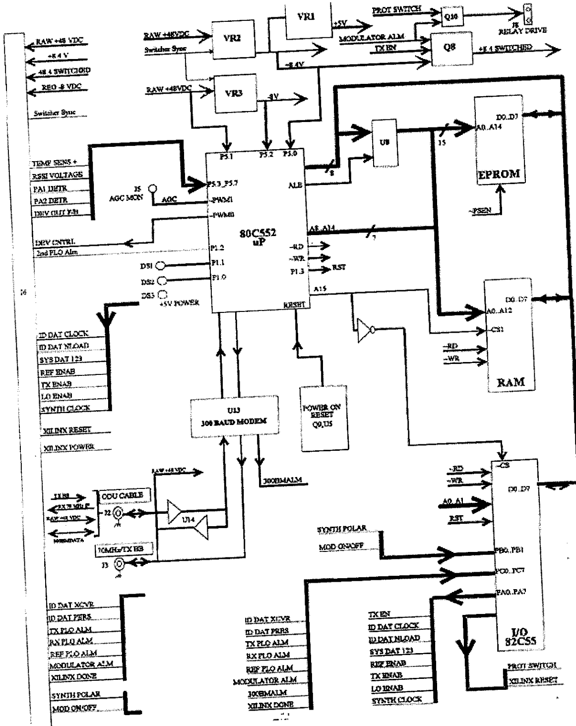
Block Diagram / CPU and Power Supply Unit
