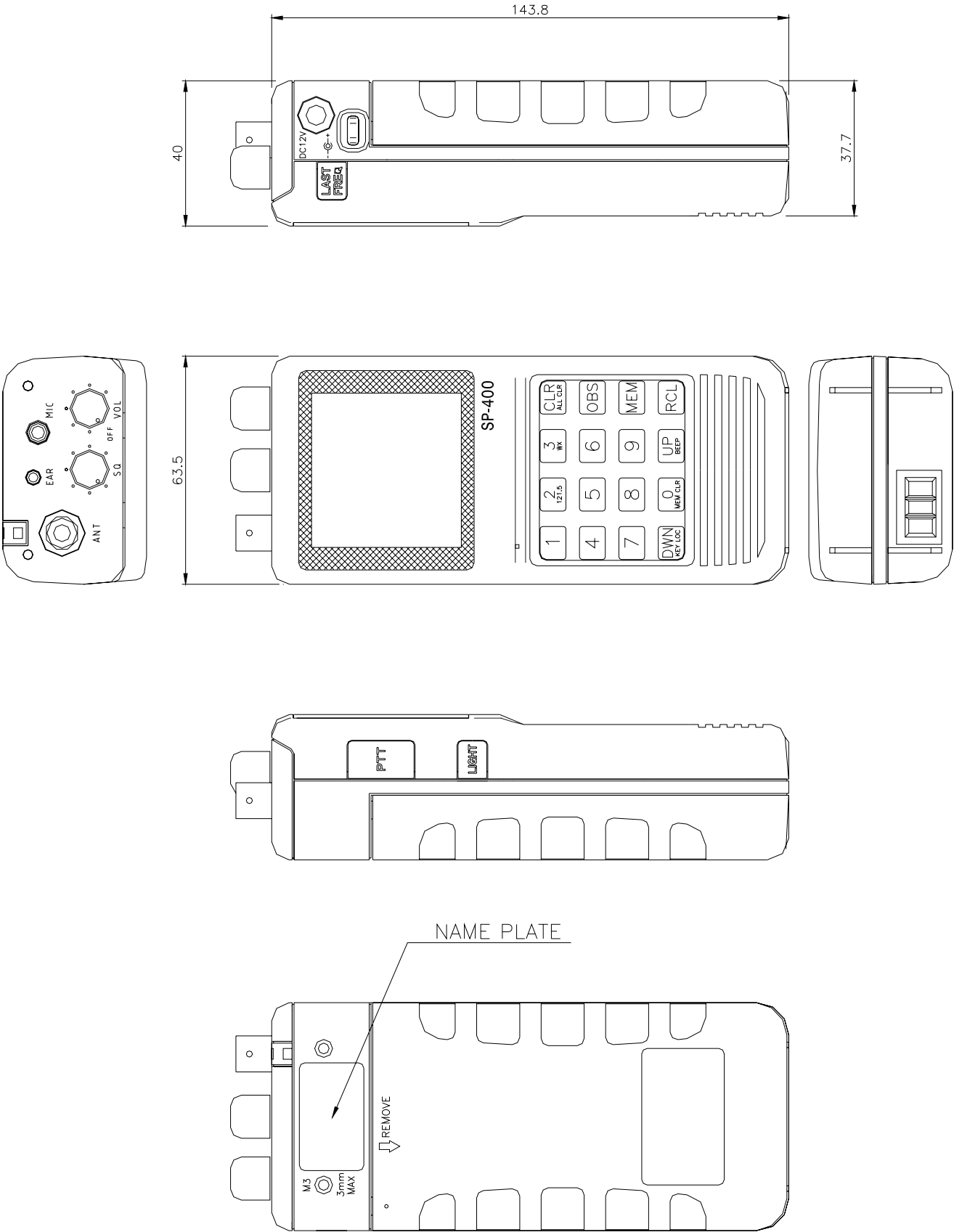
OUTLINE DRAWING OF SP-400
