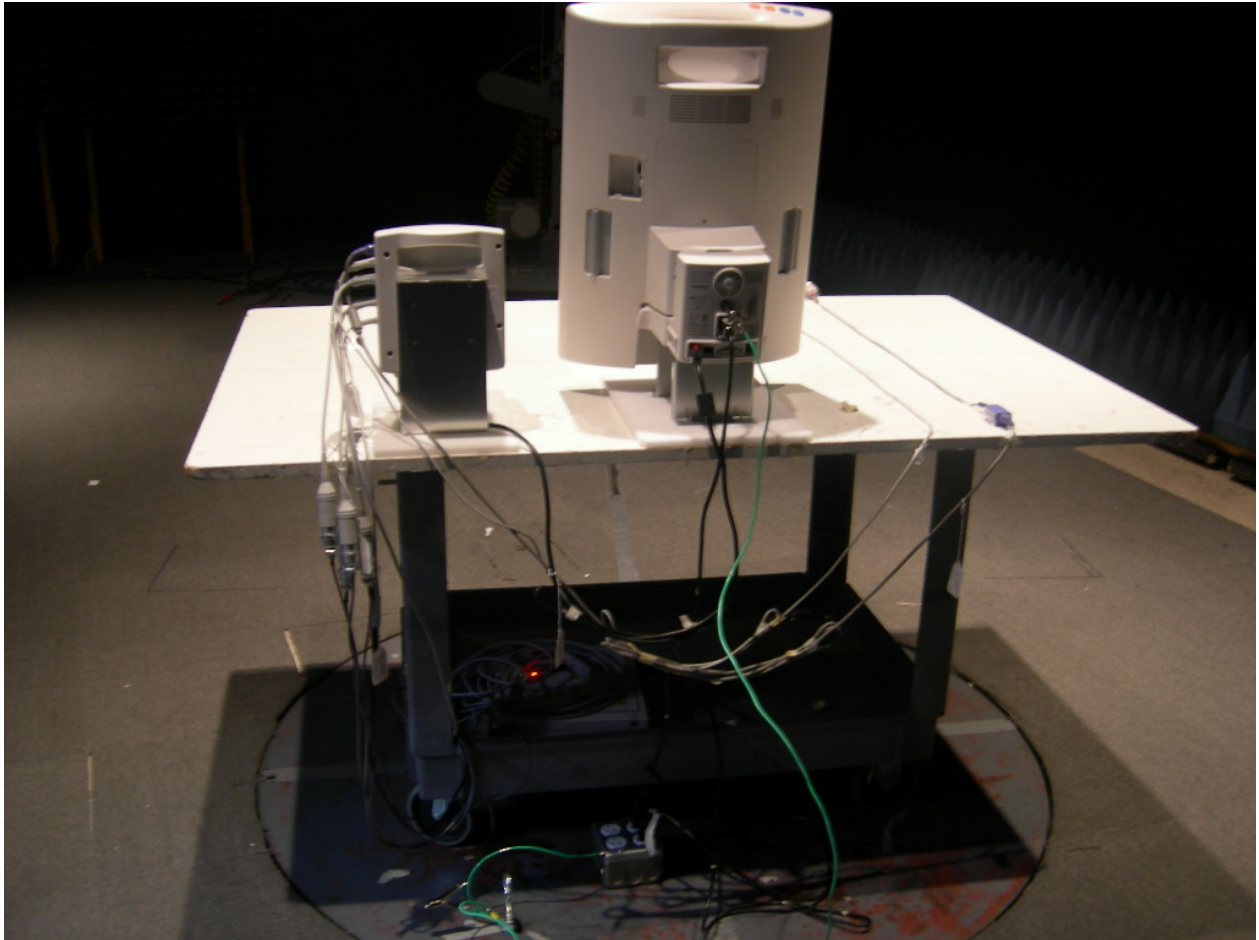
Figure 6: Radiated Emissions – V21
