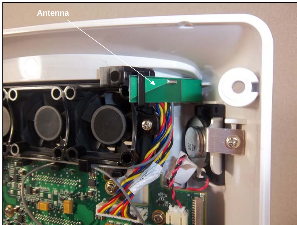
Figure 5: Internal Photo – V12
