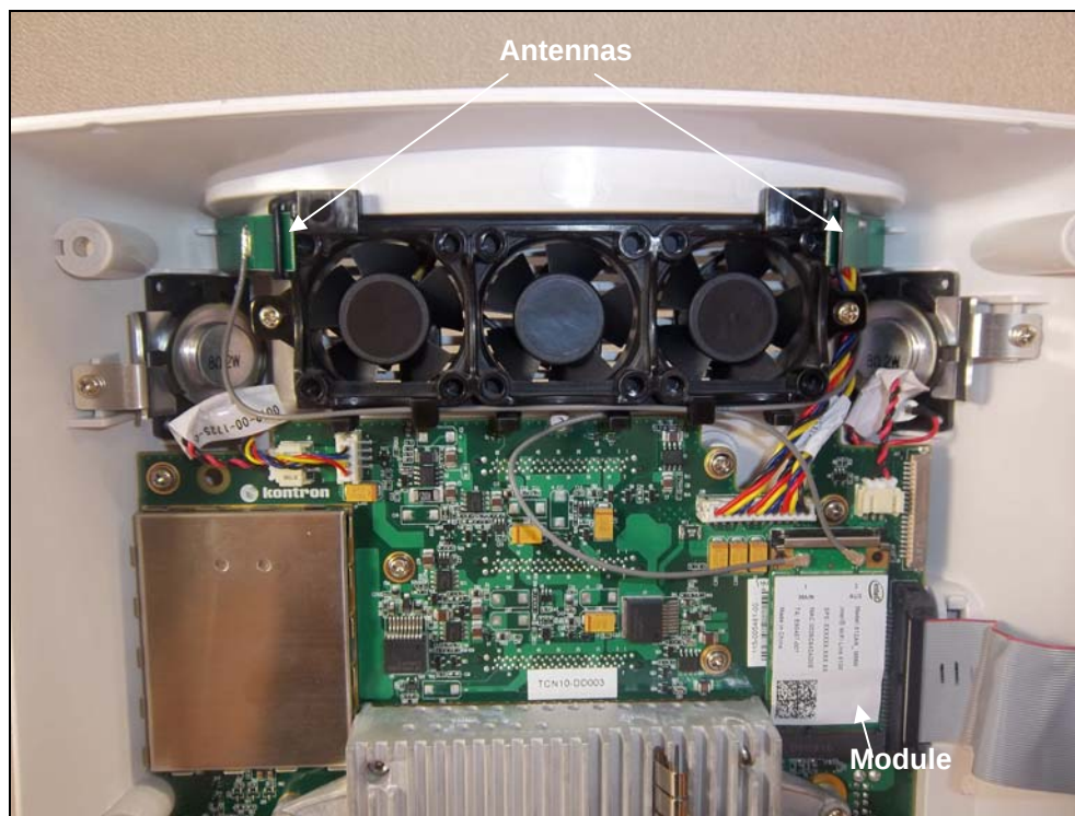
Figure 3: Internal Photo – Module inside V12
