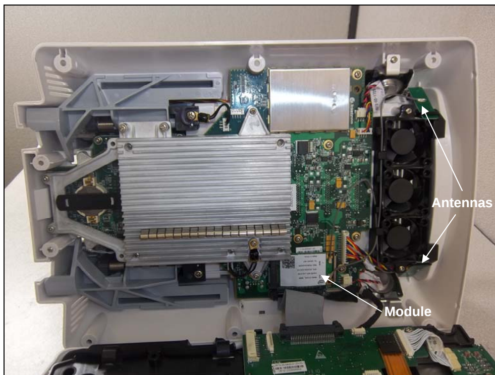
Figure 2: Internal Photo – Module inside V12
