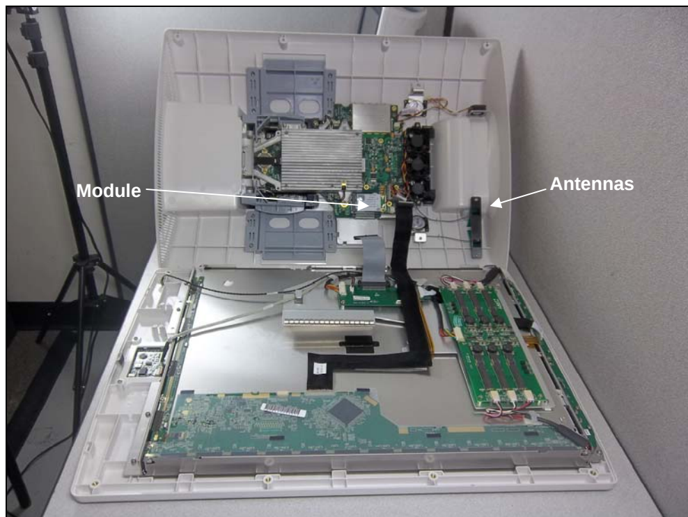
Figure 6: Internal Photo – Module inside V21
