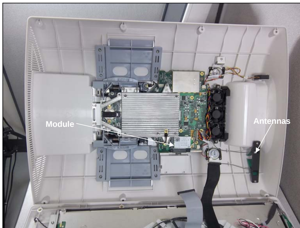
Figure 7: Internal Photo – Module inside V21
