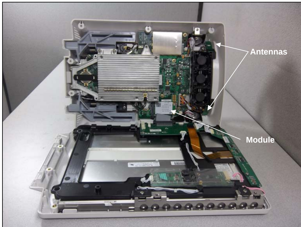
Figure 1: Internal Photo – Module inside V12
