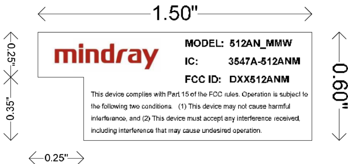
Figure 3: Label Drawing
