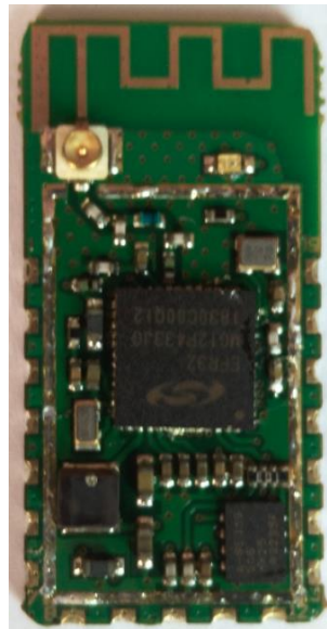
PCB Components Side & Module PCB
