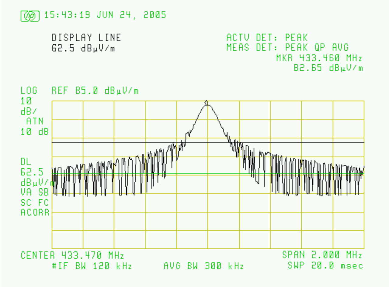
Figure 6.1 Occupied Bandwidth
