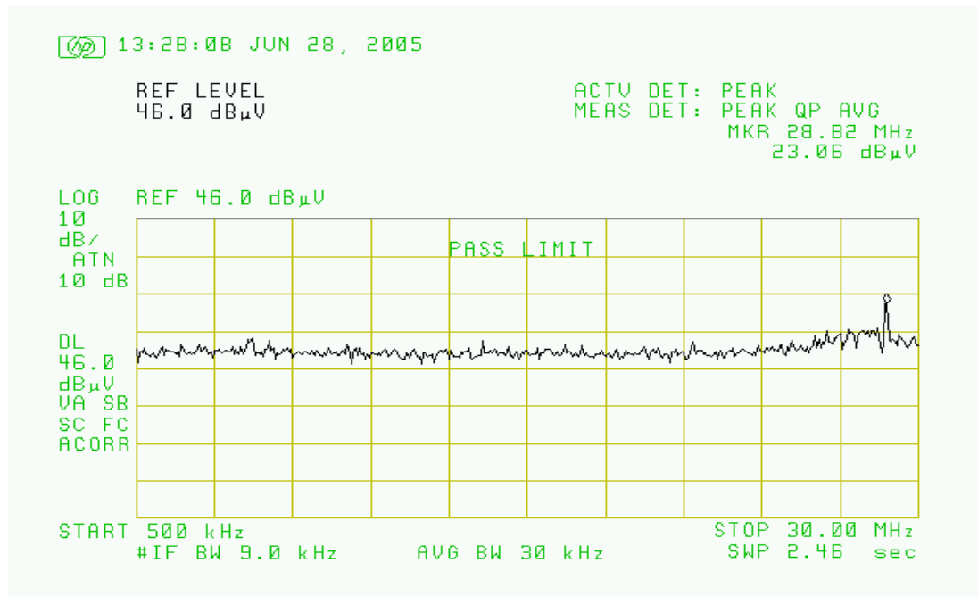
Fig. 5.1 Conducted Emission-Line
