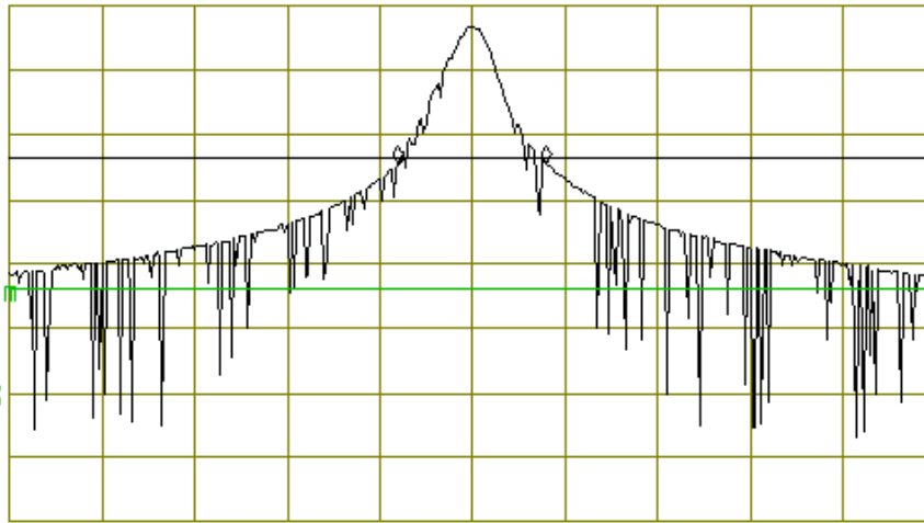
Figure 6.1 Occupied Bandwidth
