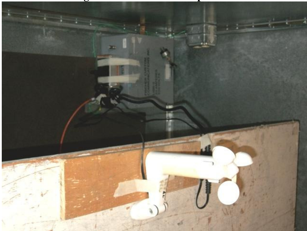
Figure 3.3 Conducted Setup- Rear
