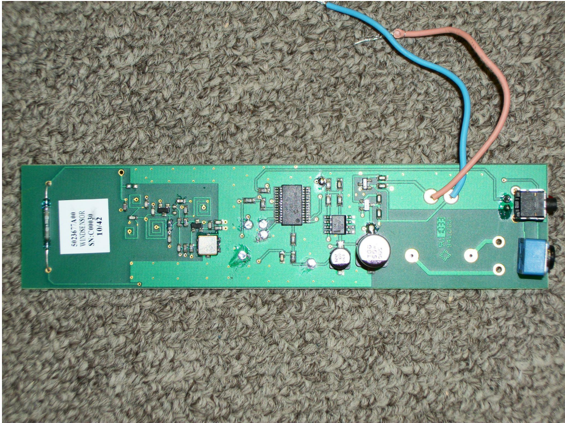
Figure 7.5 Component Side
