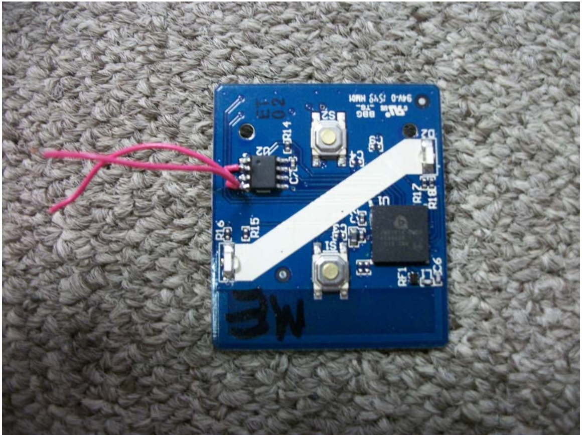
7.4 Components View
