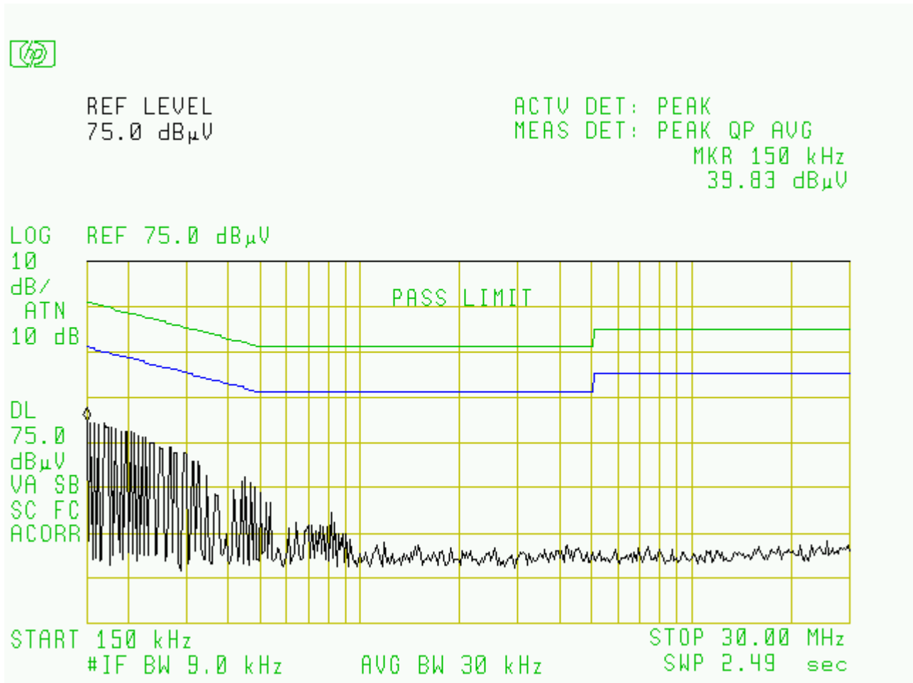
Fig. 5.2 Conducted Emission- Neutral
