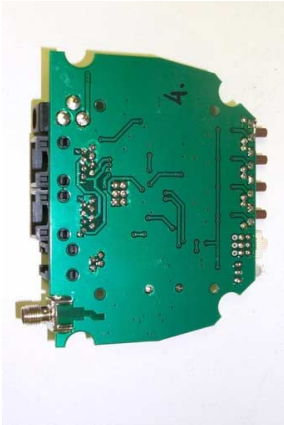
Figure 7.4 Foil Side
