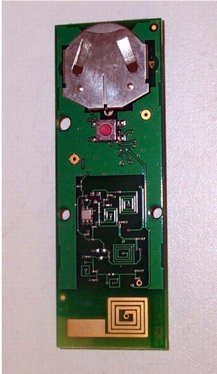
Figure 7.5 PCB Foil Side
