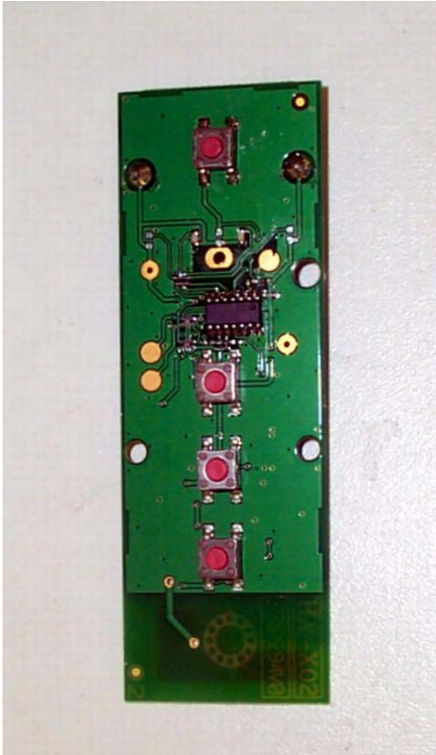
Figure 7.4 PCB Component Side
