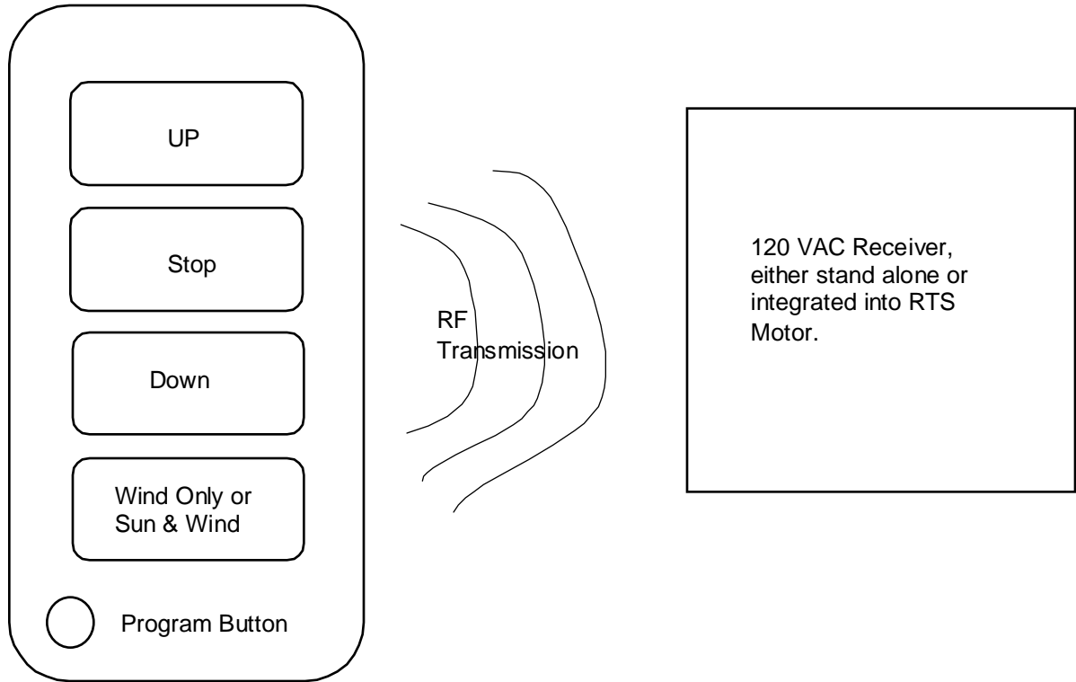
Telis Soliris Handheld Transmitter
