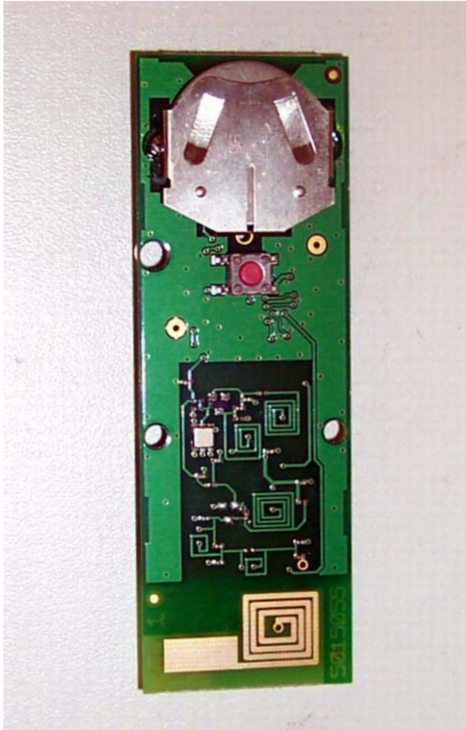
Figure 7.5 PCB Foil Side
