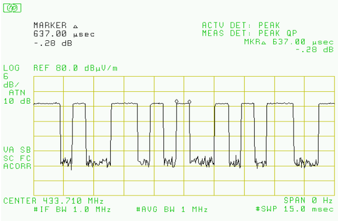
Figure 6.2 (b) Pulse Train Timing
