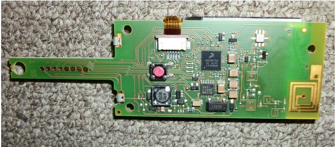
Figure 7.5 Component Side
