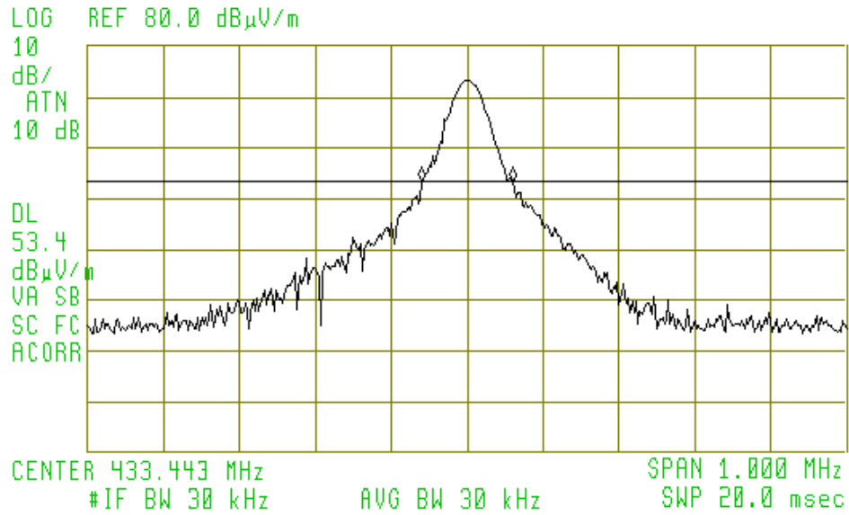
Figure 6.1 Occupied Bandwidth
