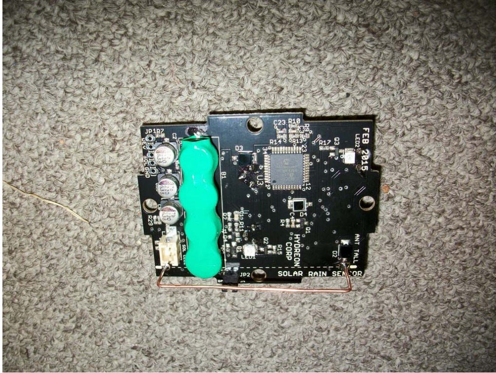
Figure 7.5 Foil Side
