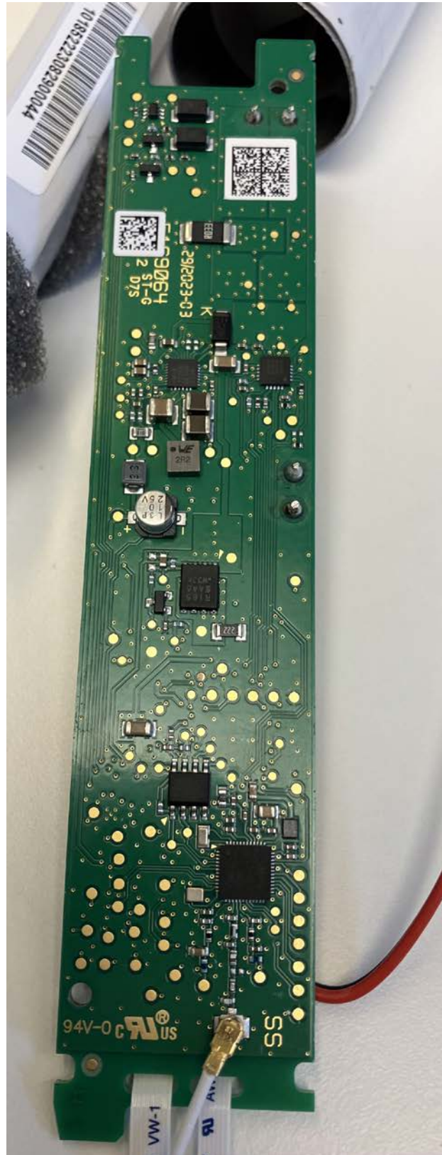
EUT Main PCB Back
