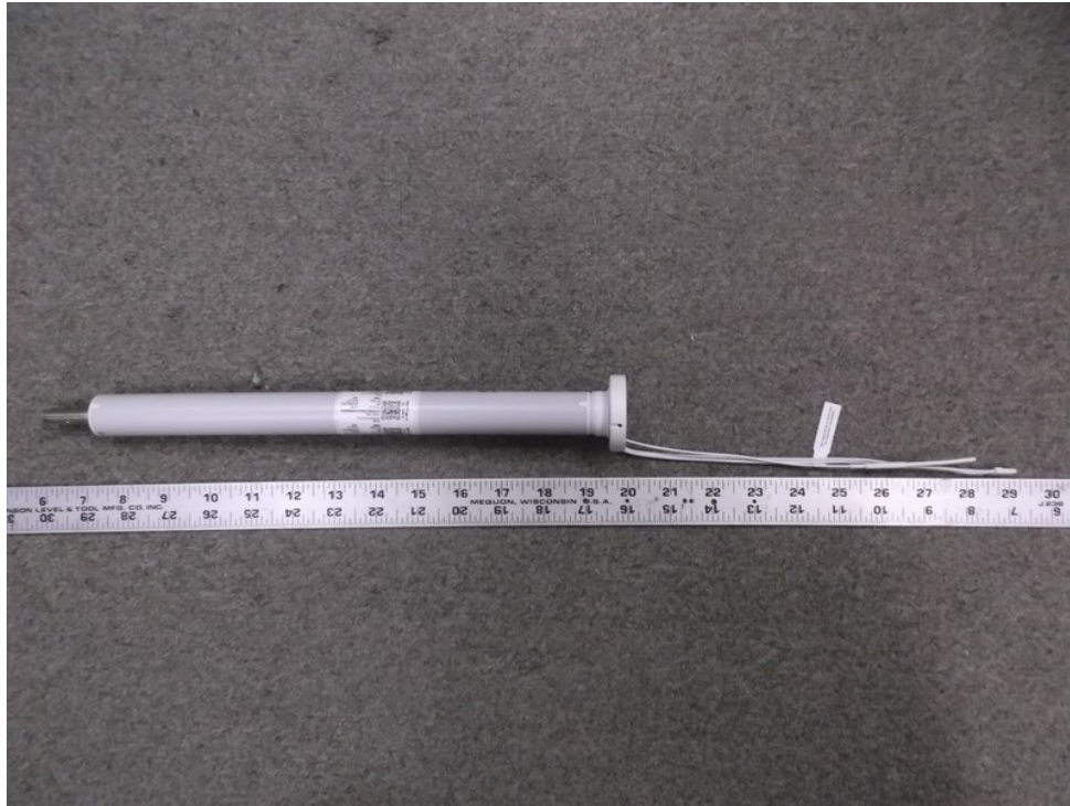
EUT- 1241672 Top View & Dimension
