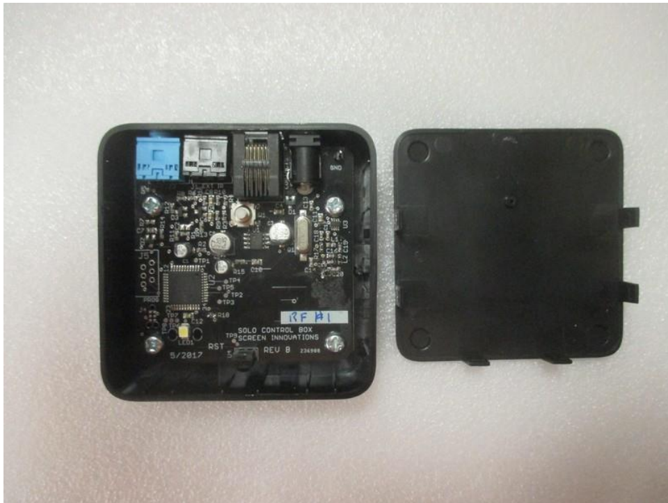
Figure 7.6 EUT Inside View
