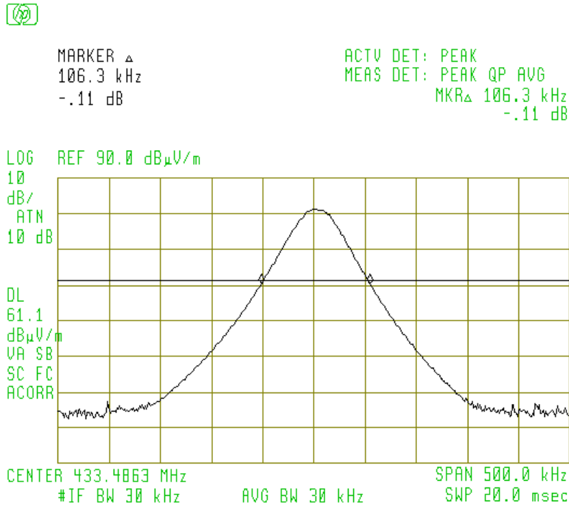
Figure 6.1 Occupied Bandwidth
