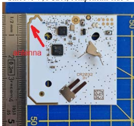
Smoove 4 , PCBA, components side 1
