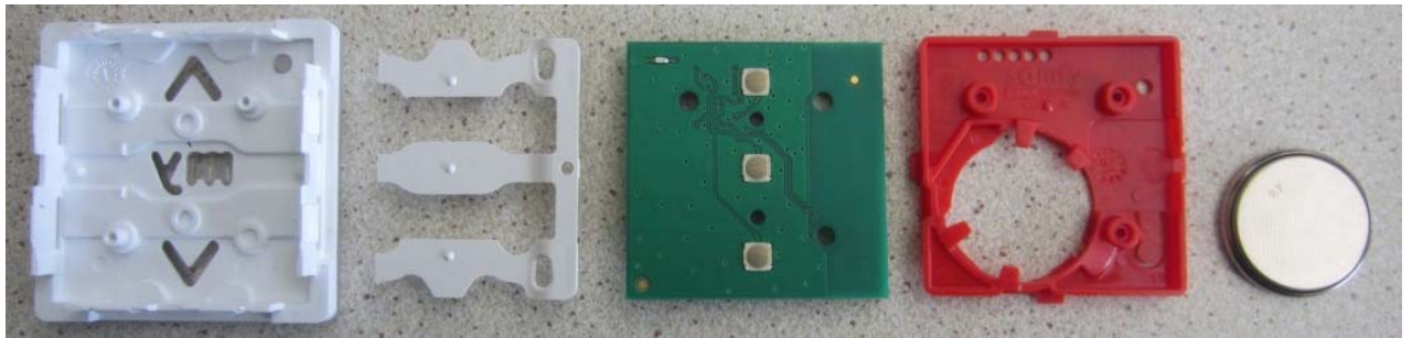
Figure 7.3 Inside View
