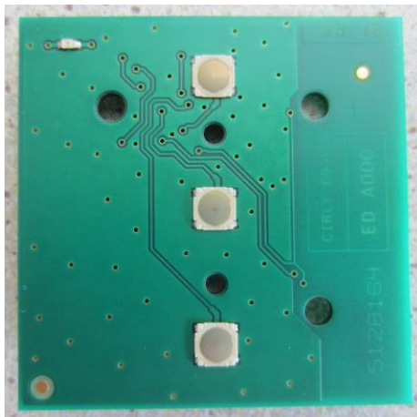
Figure 7.5 Foil Side
