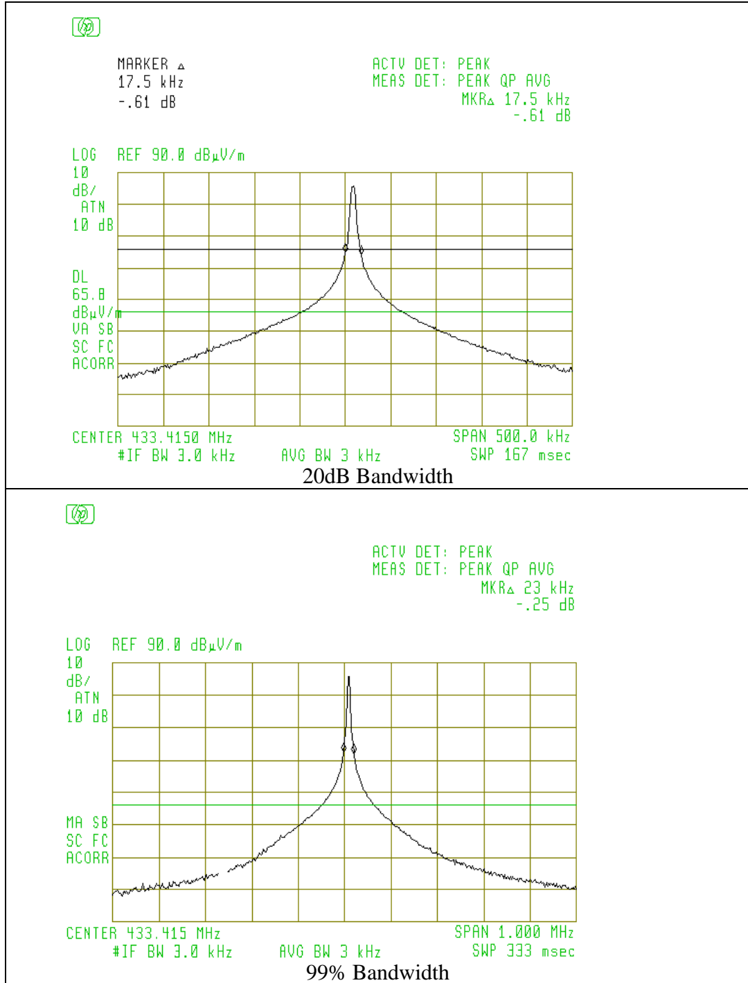
Figure 6.1 Occupied Bandwidth
