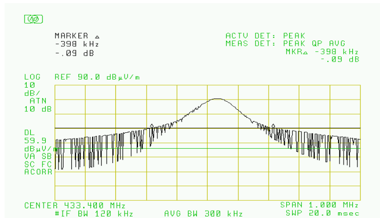
Figure 6.1 Occupied Bandwidth
