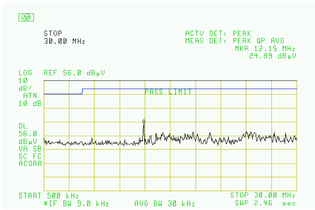
Fig. 5.1 Conducted Emission-Line
