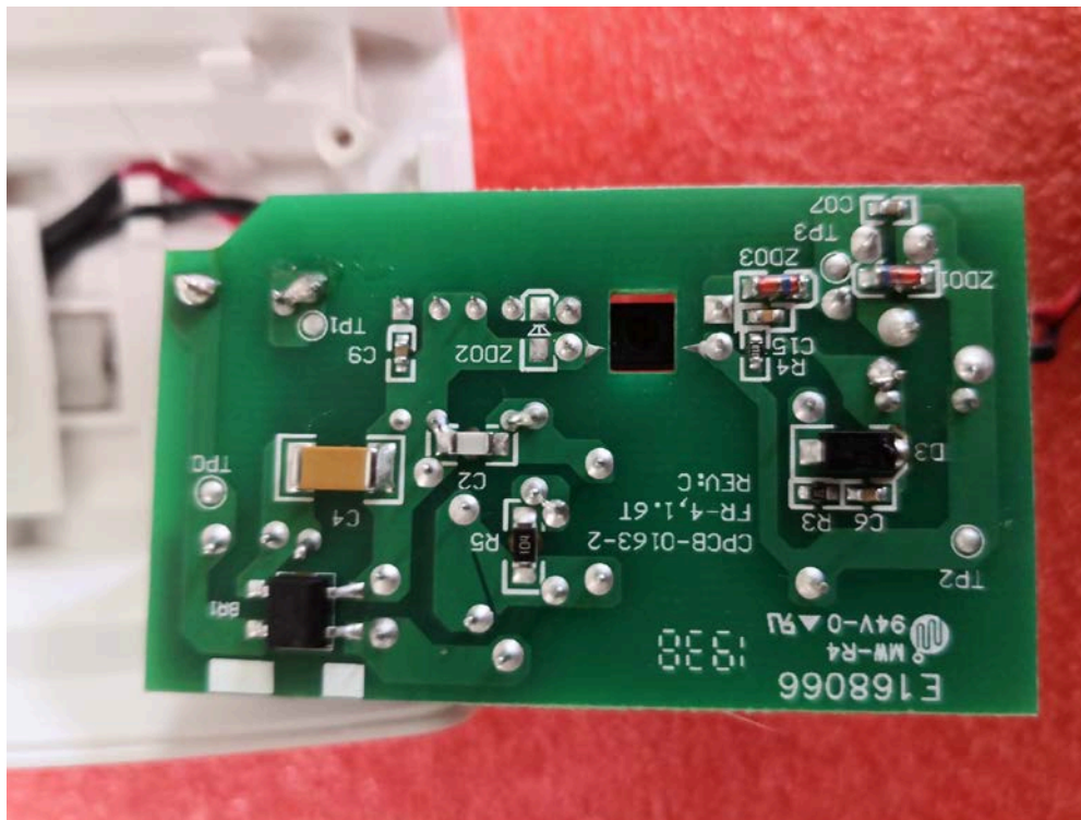
Figure 7.11 Power Supply Board Foil Side
