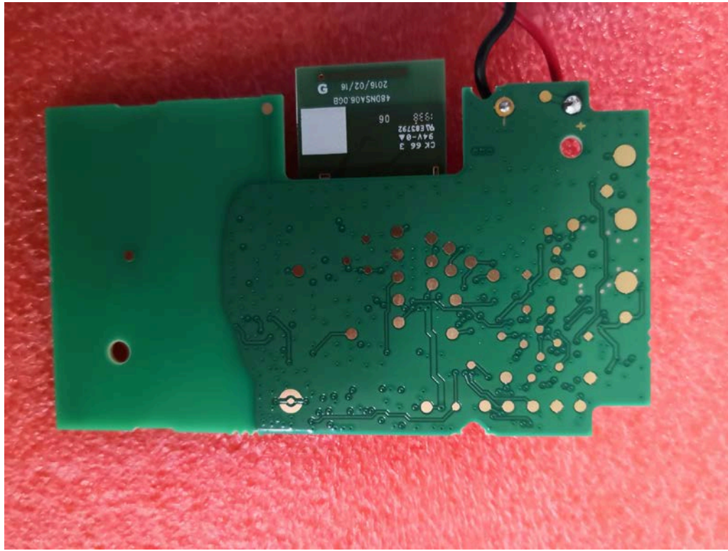
Figure 7.10 RF Board Foil Side
