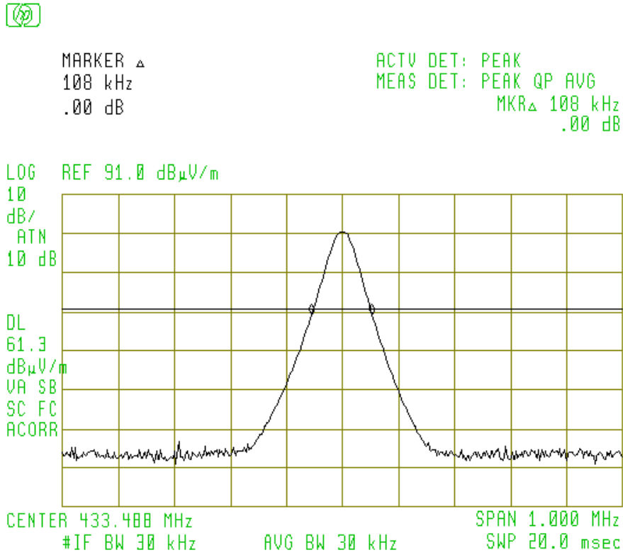
Figure 6.1 Occupied Bandwidth
