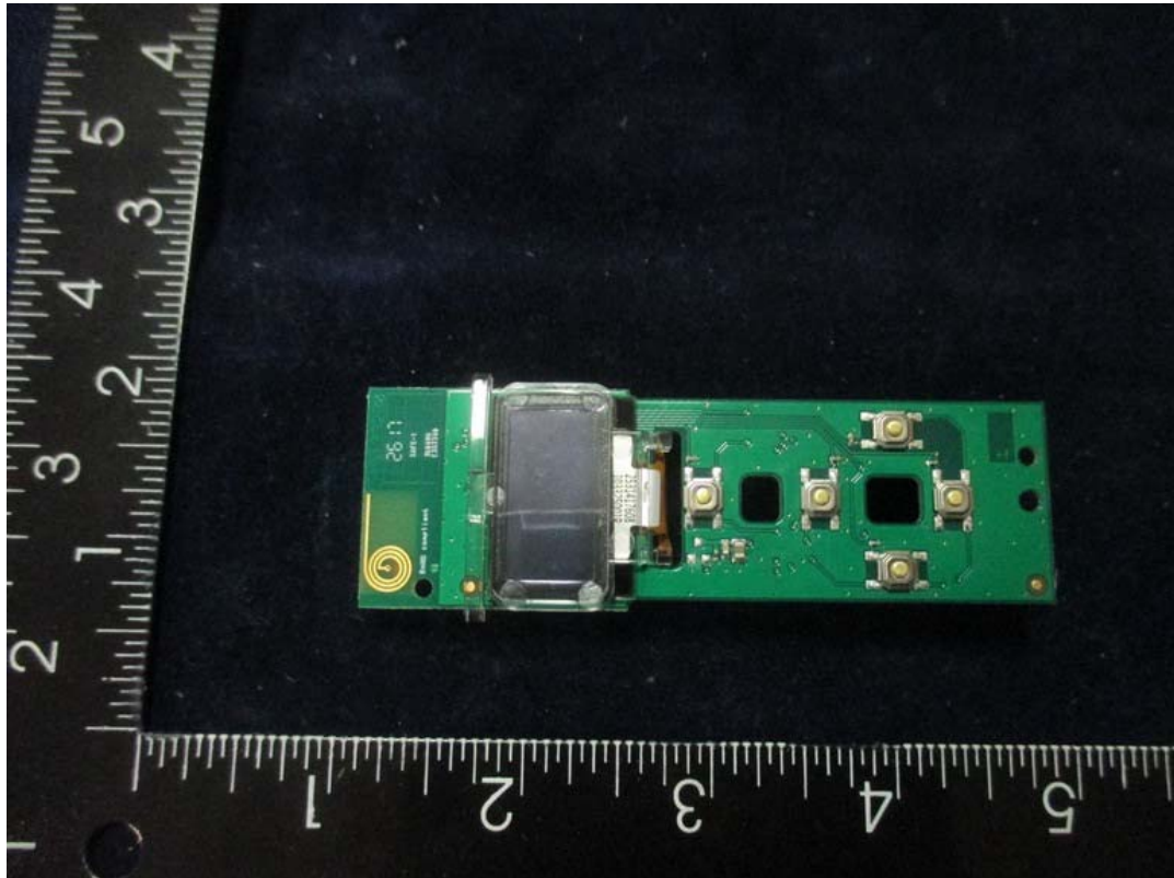
7.8 Foil Side View
