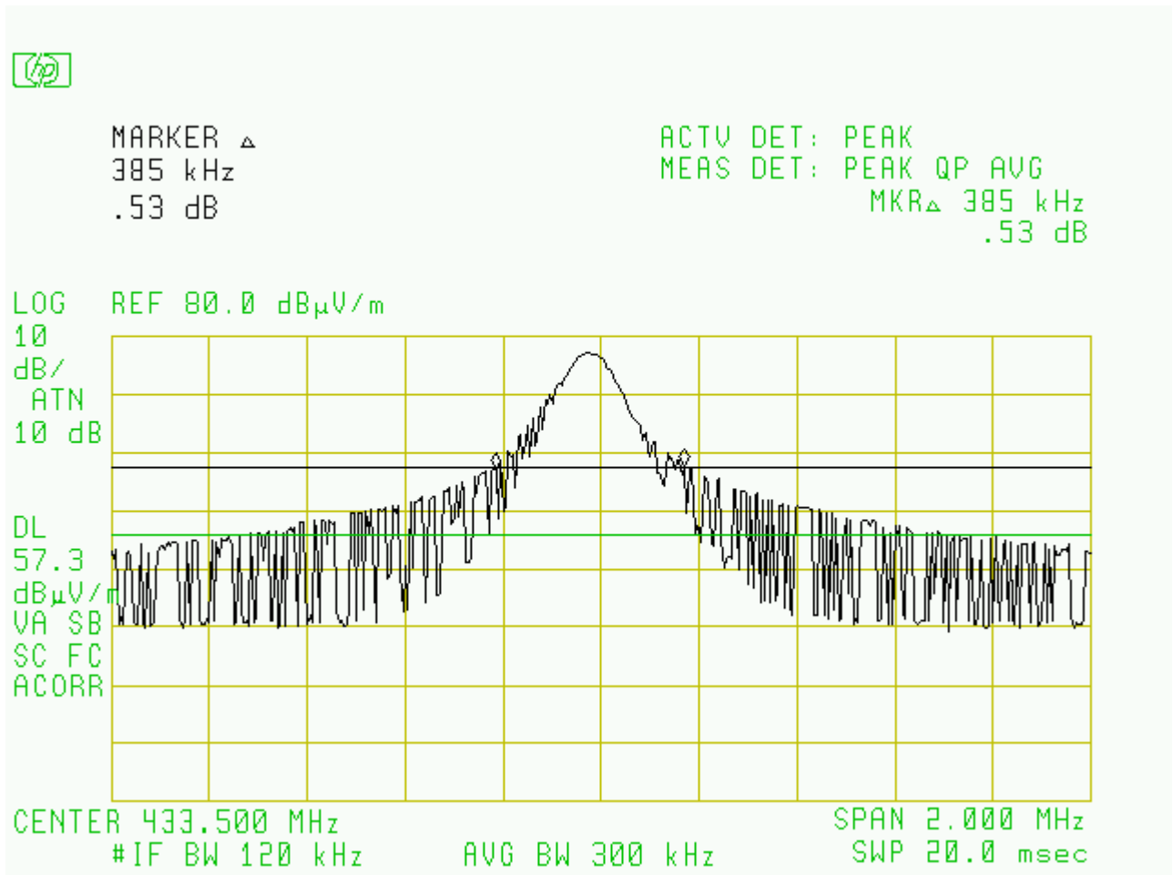
Figure 6.1 Occupied Bandwidth
