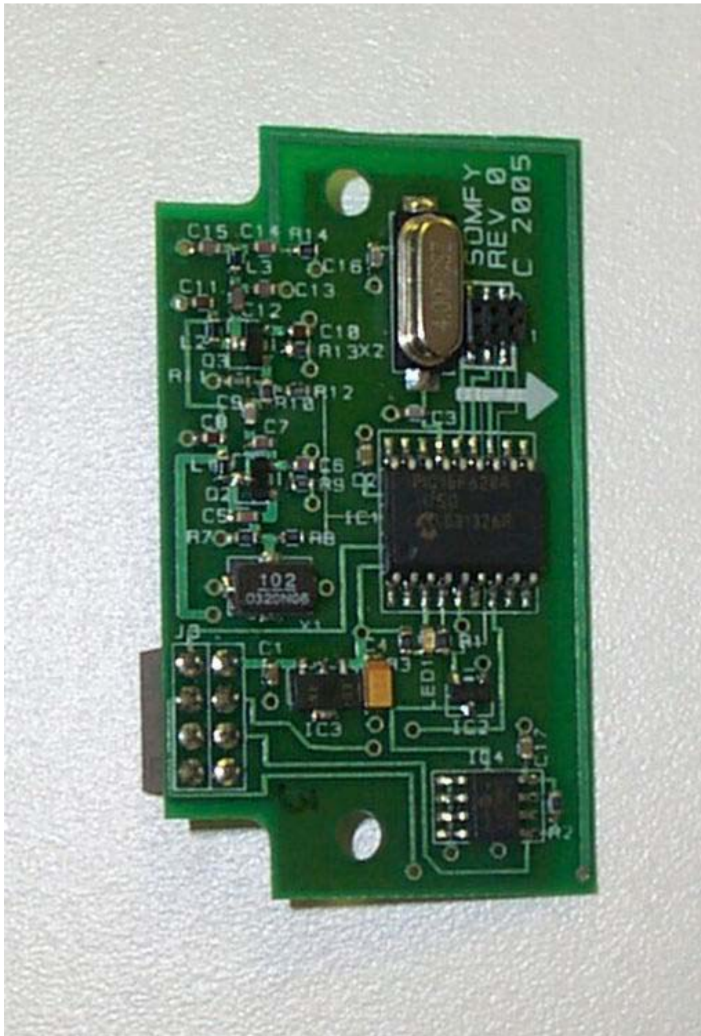
Component Side
