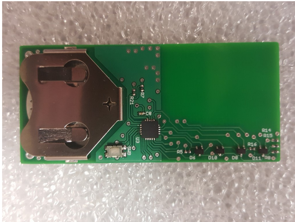
Figure 7.6 Foil Side
