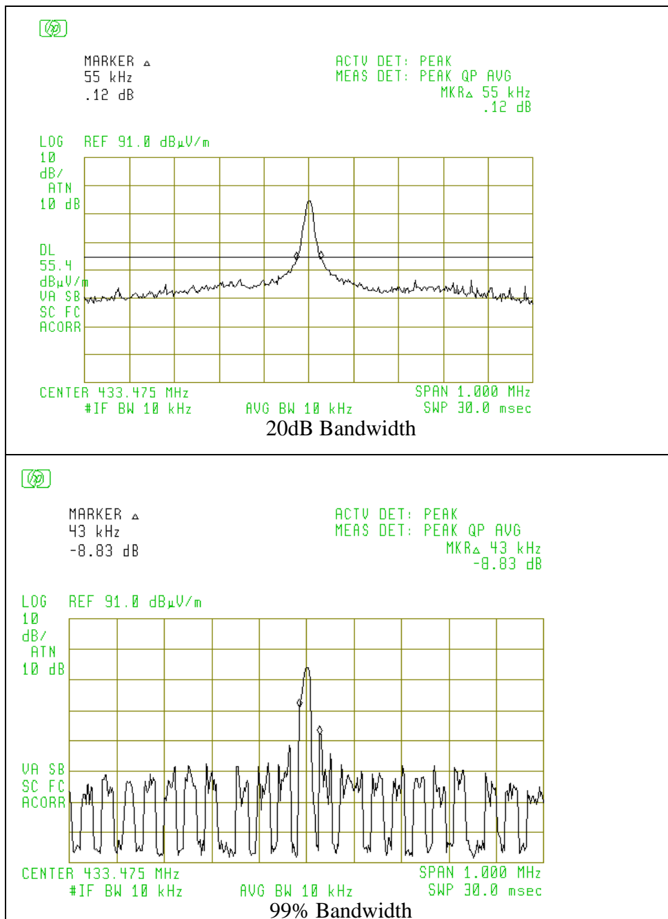
Figure 6.1 Occupied Bandwidth
