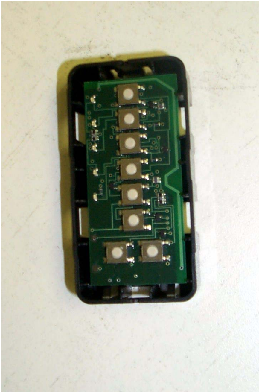
Figure 7.4 Foil Side
